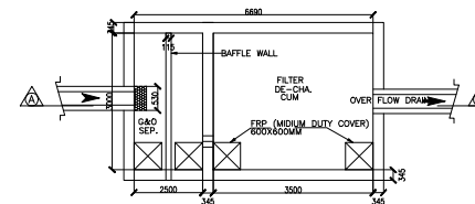
TYPICAL PLAN OF RAIN WATER HARVESTING
