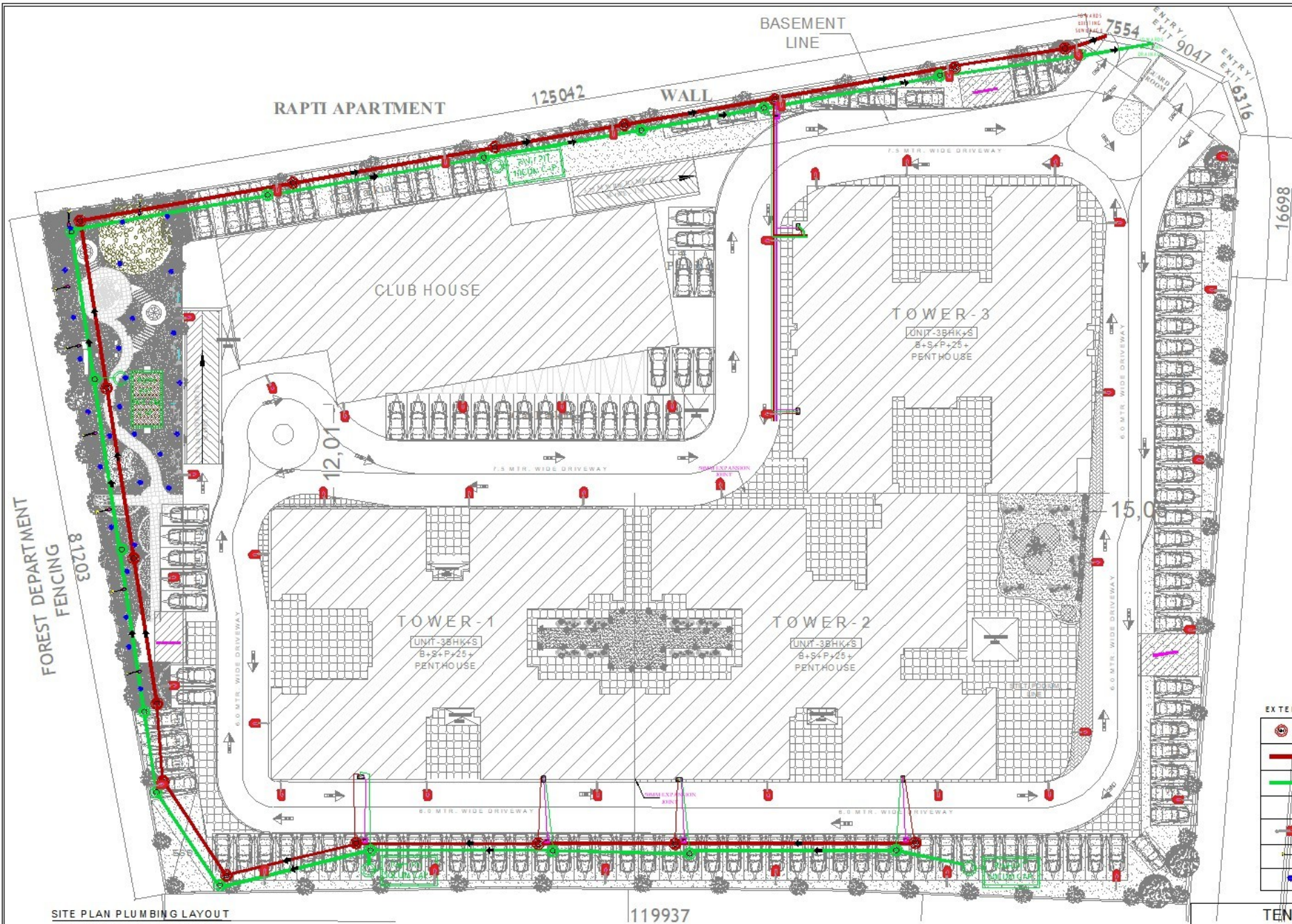
SITE PLAN PLUMBING LAYOUT
