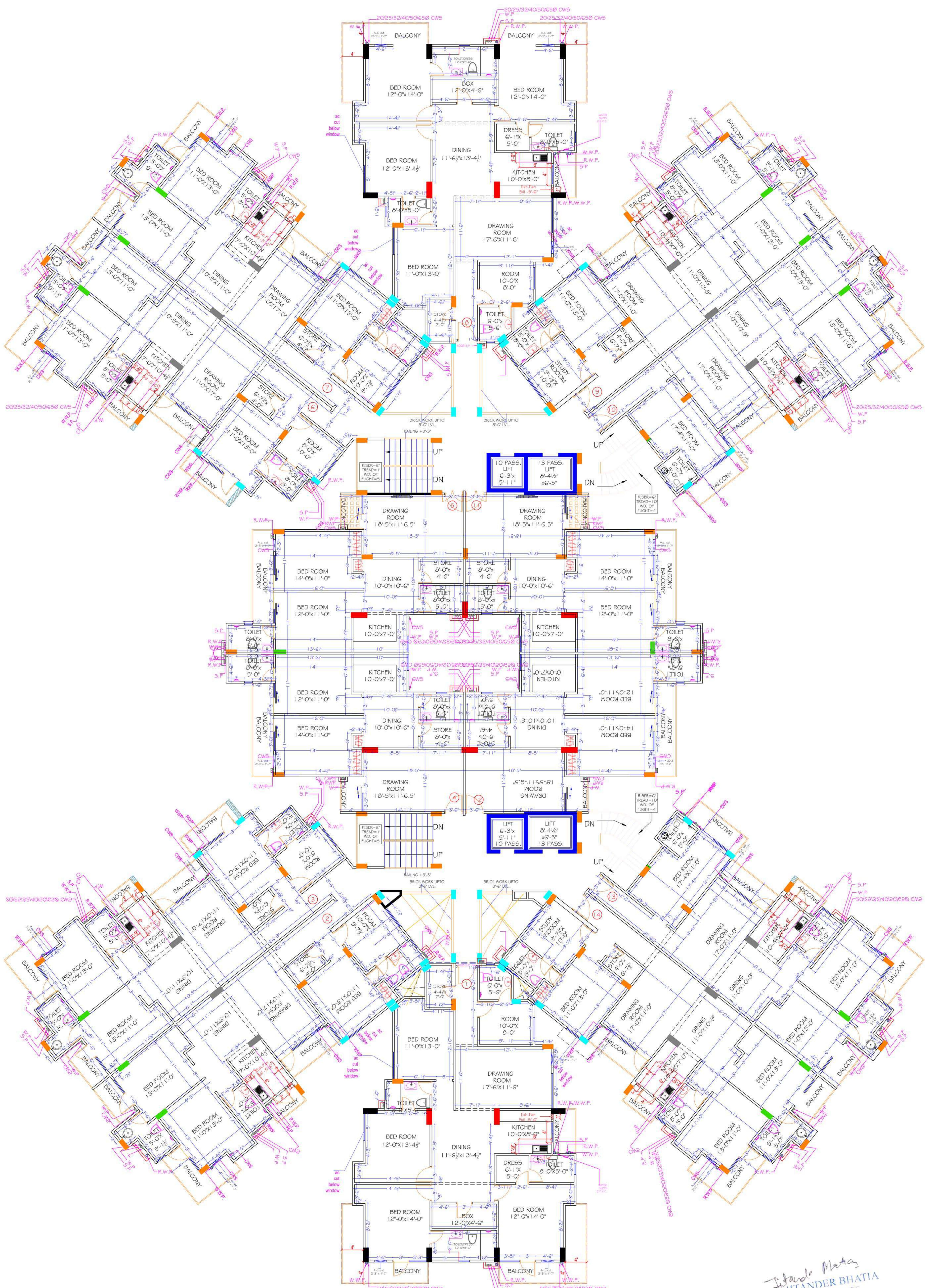
TYPICAL FLOOR PLAN
