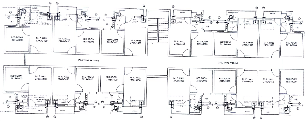
TYPICAL FLOOR PLAN G+3 (SANITARY)
