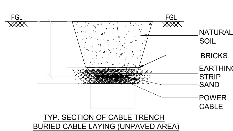
TYP. SECTION OF CABLE TRENCH BURIED CABLE LAYING (UNPAVED AREA)
