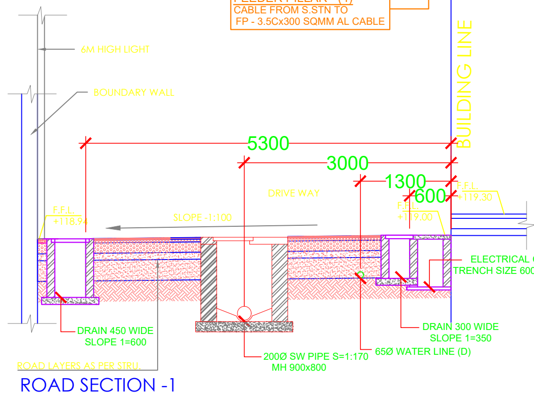
ROAD SECTION - I
