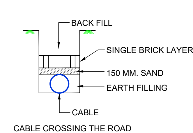
CABLE CROSSING THE ROAD
