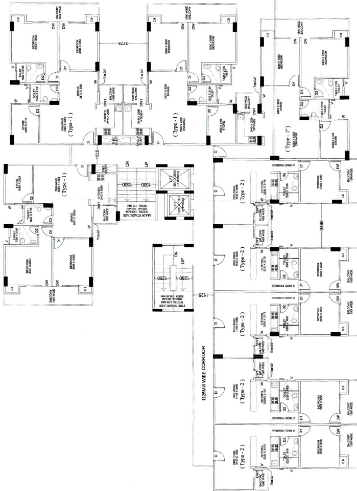
2nd to 13th FLOOR PLAN
