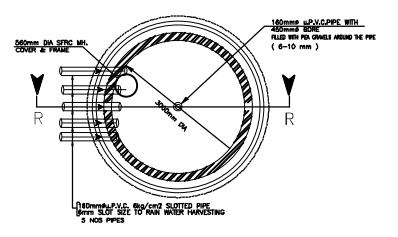
SECTION DETAIL OF DESILTING CHAMBER RAIN WATER HARVESTING ( RECHARGE SHAFT ) 3000 mm DIA & 3000 mm (EFFECTIVE DEPTH)
