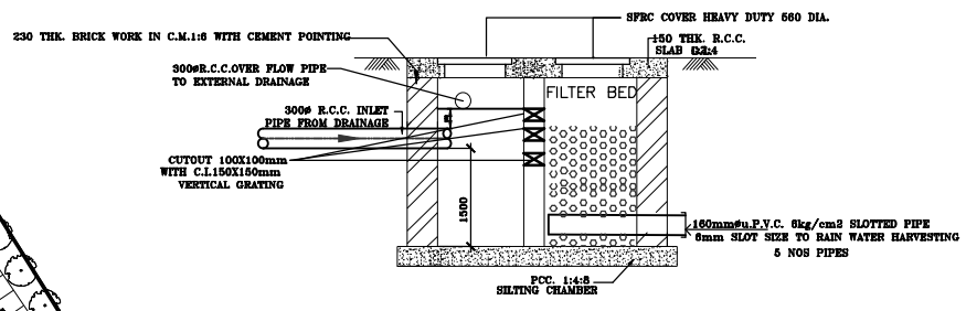
SECTION-AA DESILT CHAMBER DETAILS 3000X1500X500mm (EFFECTIVE DEPTH)
