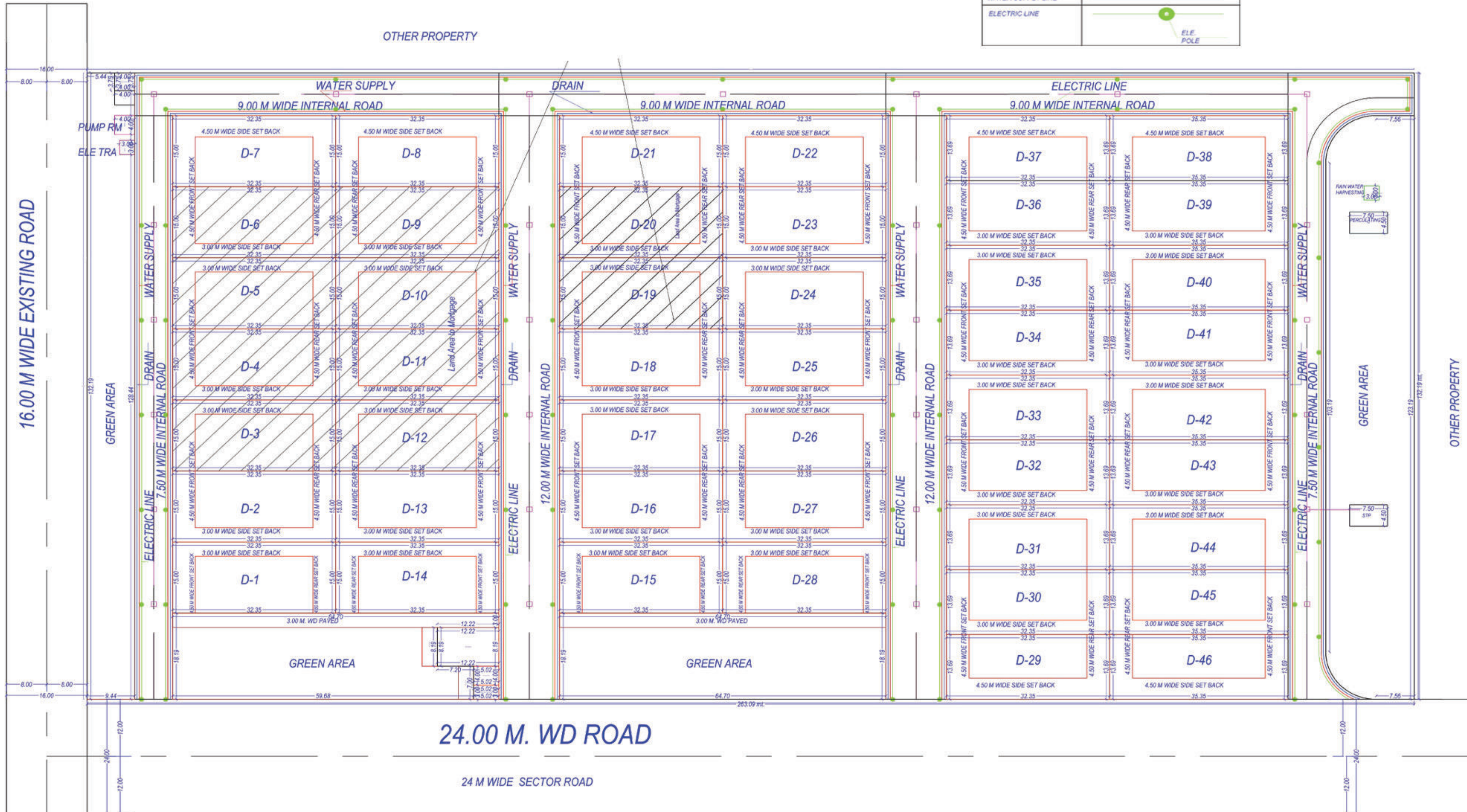
WATER SUPPLY PLAN
