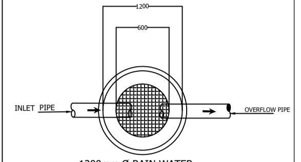
1200mm Ø RAIN WATER PERCOLATION PIT (SCALE : NTS)
