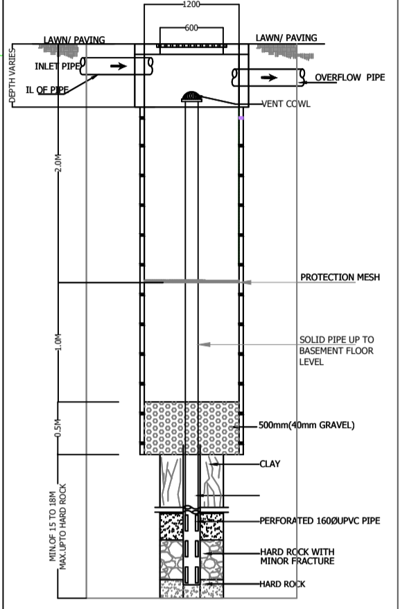
SECTIONAL DETAIL (SCALE: NTS)
