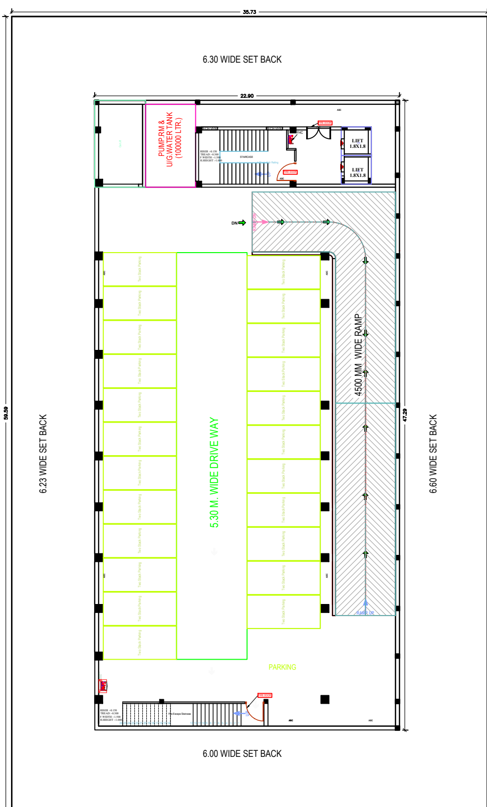
LOWER BASEMENT FLOOR PLAN SCALE 1:100
