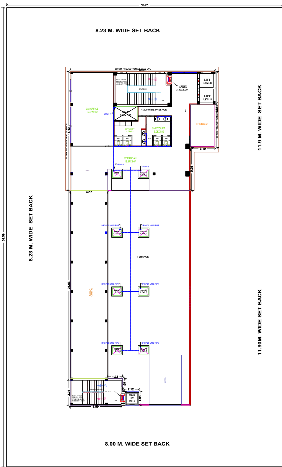
SIXTH FLOOR PLAN SCALE 1:100
