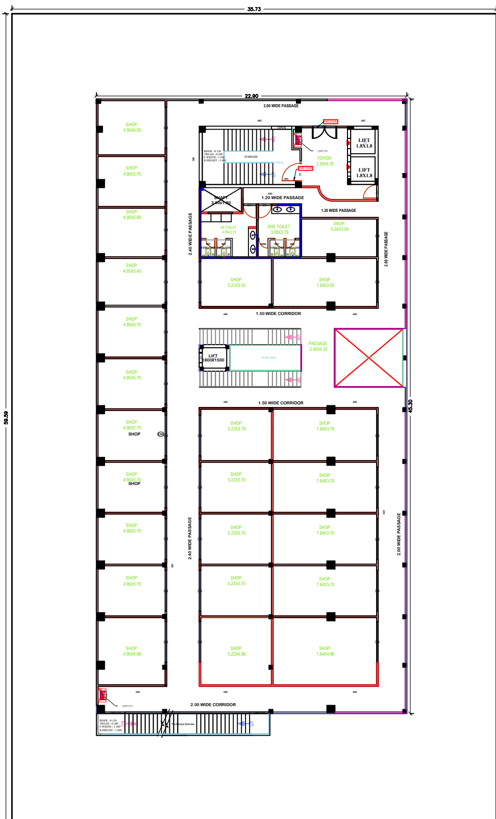
SECOND FLOOR PLAN SCALE 1:100
