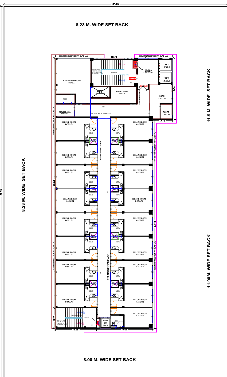
FOURTH FLOOR PLAN SCALE 1:100
