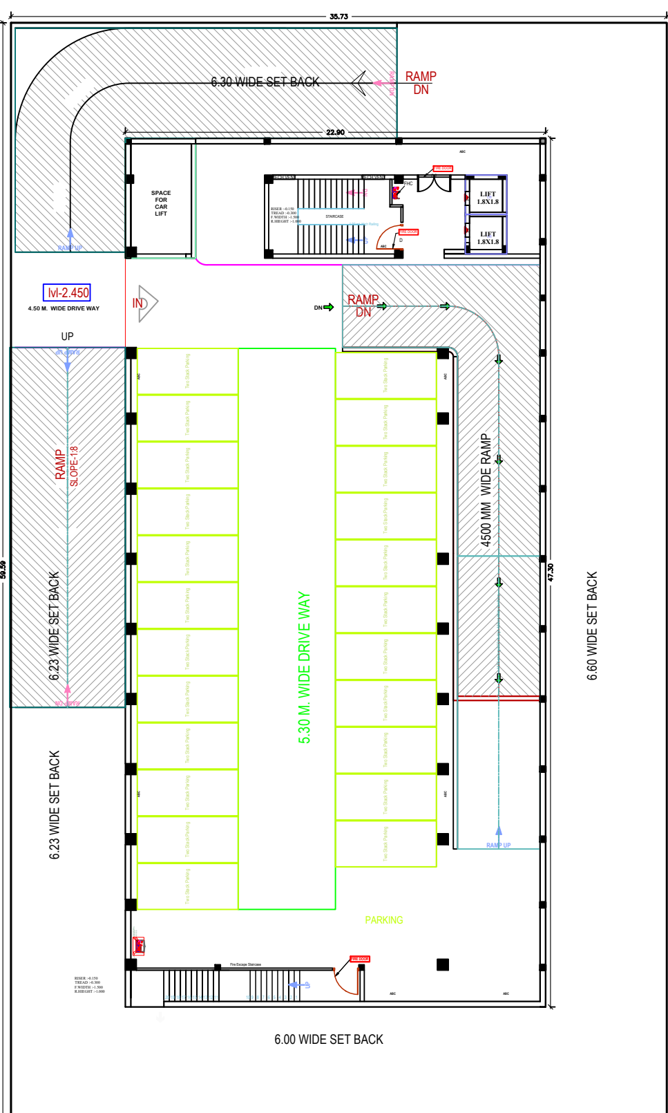
UPPER BASEMENT FLOOR PLAN SCALE 1:100
