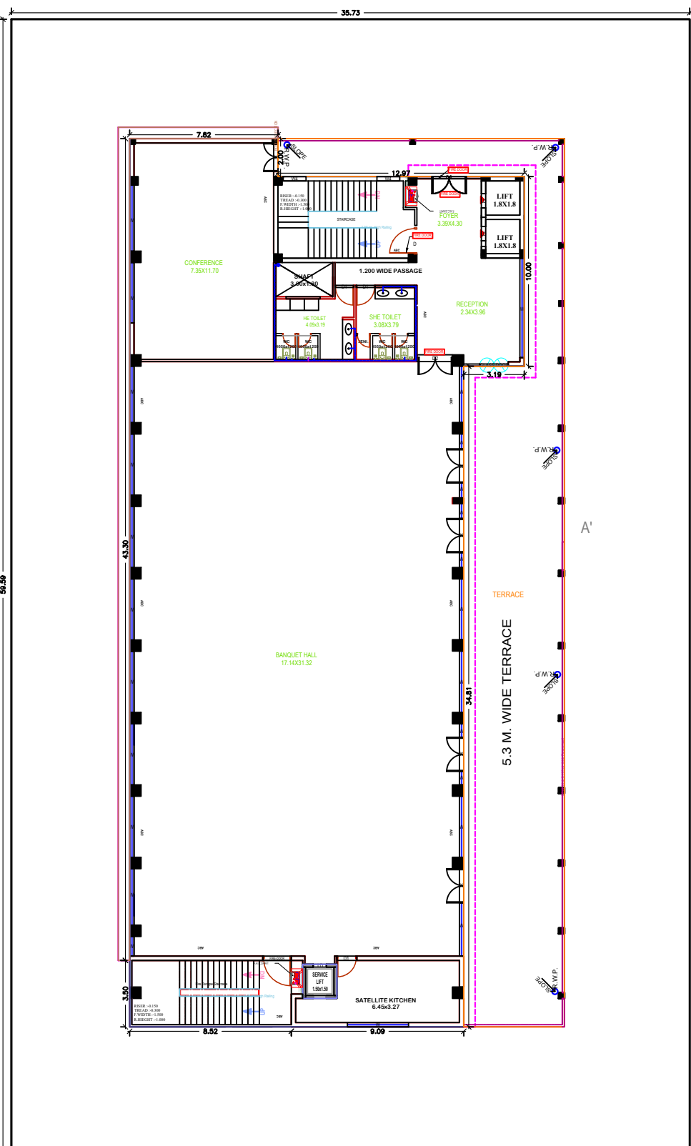
THIRD FLOOR PLAN SCALE 1:100
