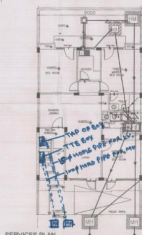
SERVICES PLAN SCALE 1:100 (ELECTRICAL LAYOUT PLAN)
