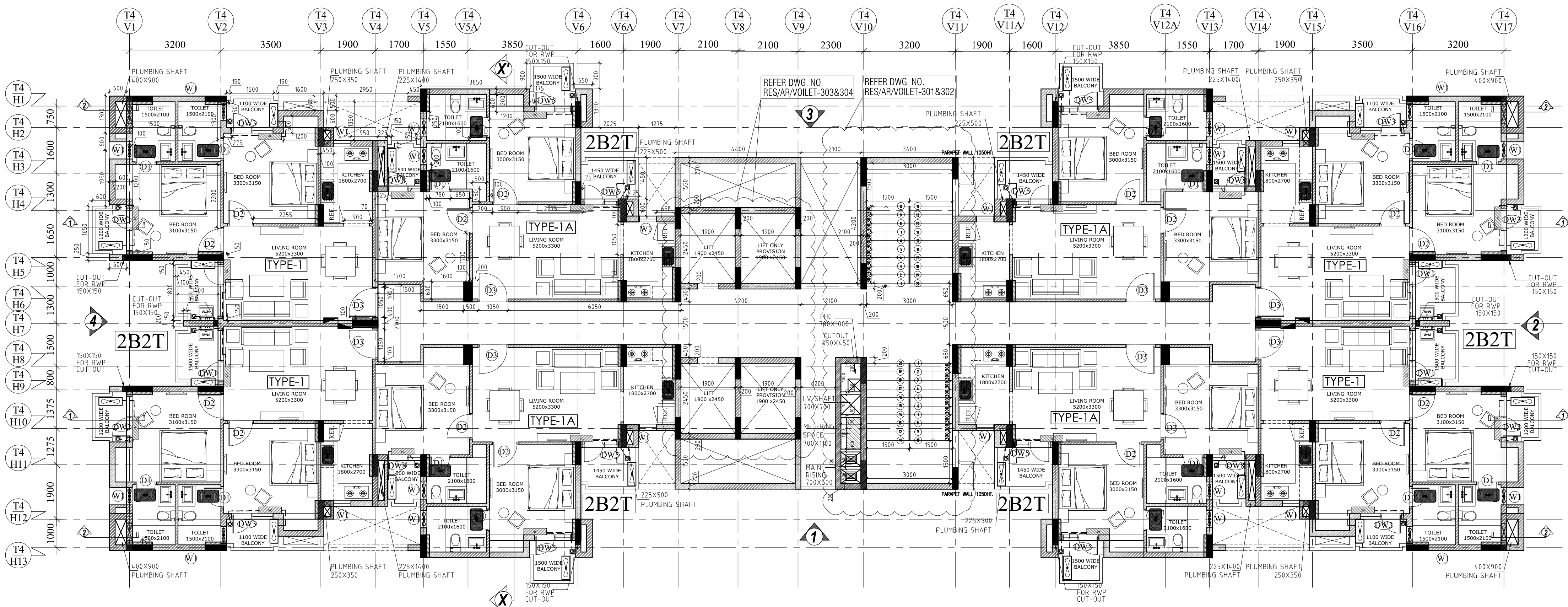
TYPICAL LEVEL FLOOR PLAN FOR PODIUM,1ST, 2ND, 7TH, 8TH, 13TH & 14TH FLOOR
