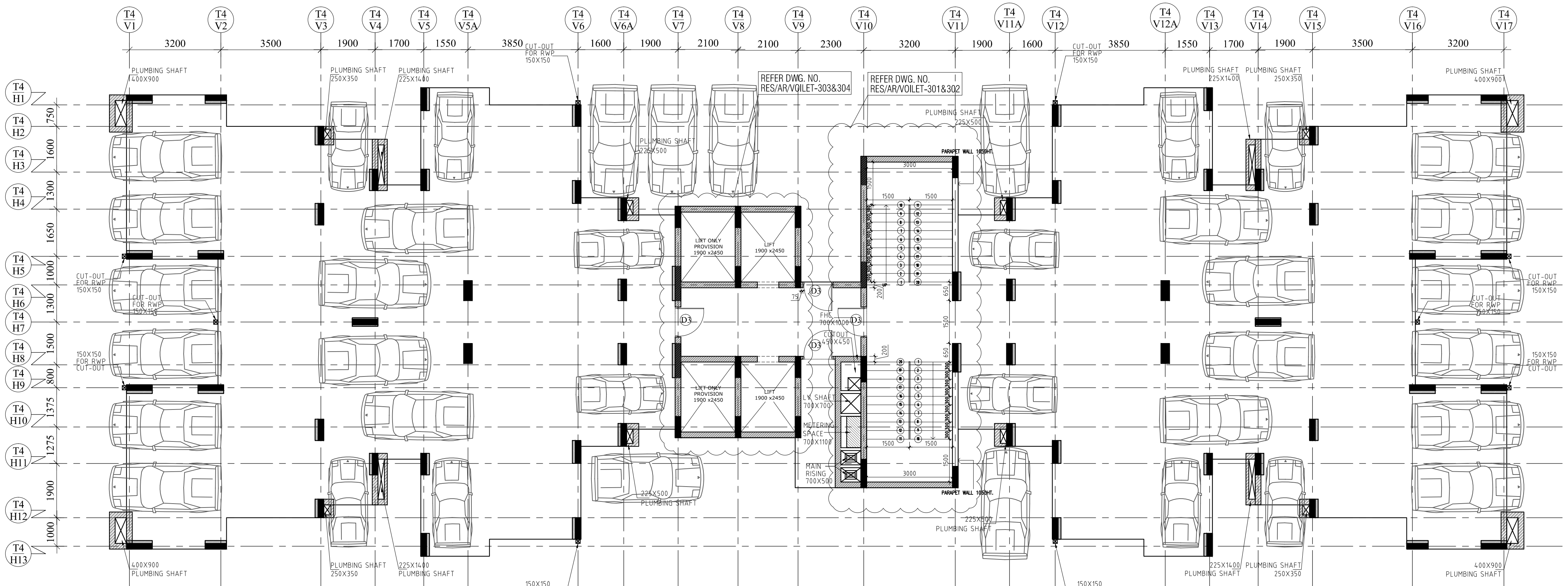
STILT LEVEL FLOOR PLAN
