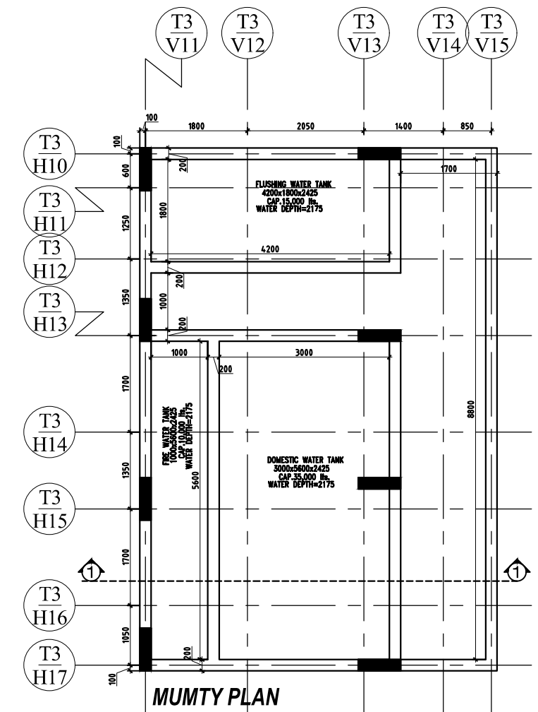
MUMTY PLAN
