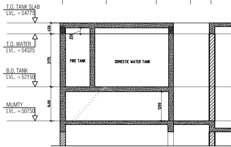
SECTION AT 1-1
