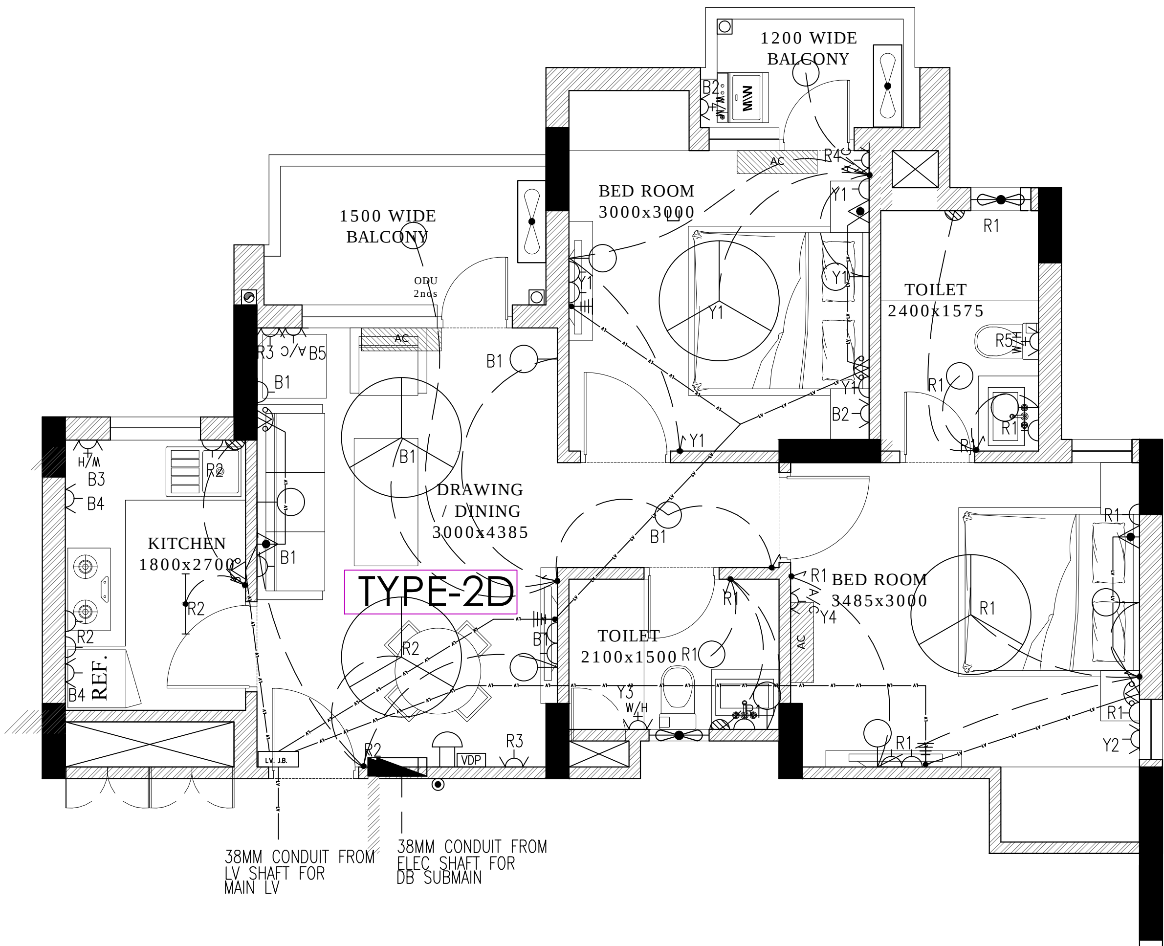
TYPICAL TYPE 2 D FLAT ELECTRICAL LAYOUT
