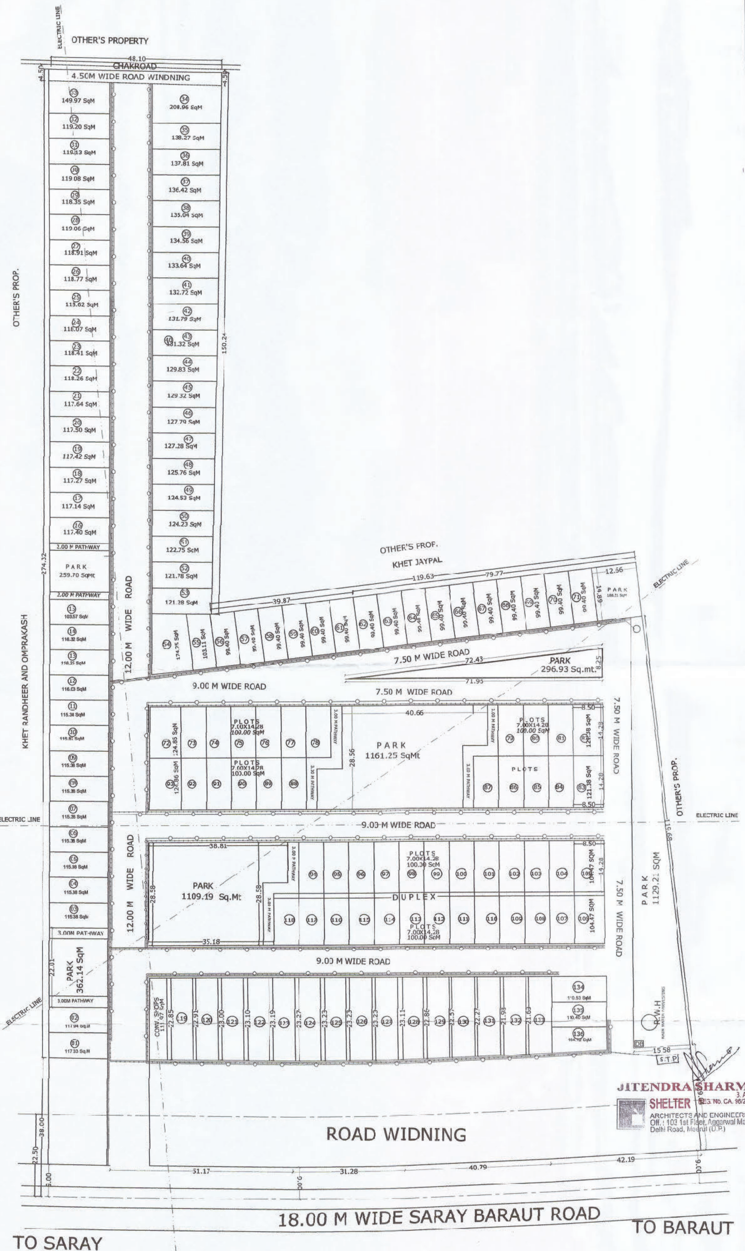
SEWER PLAN SCALE:- 1:500
