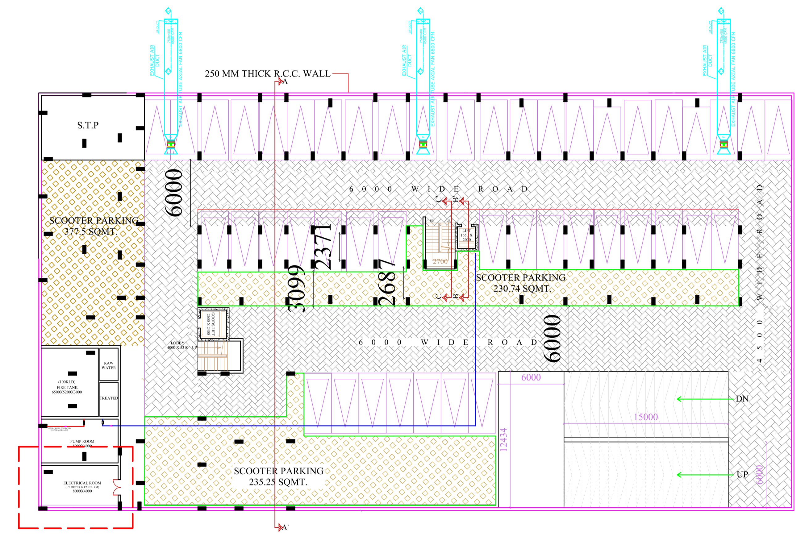
1st & 2nd BASEMENT FLOOR PLAN SCALE 1:200
