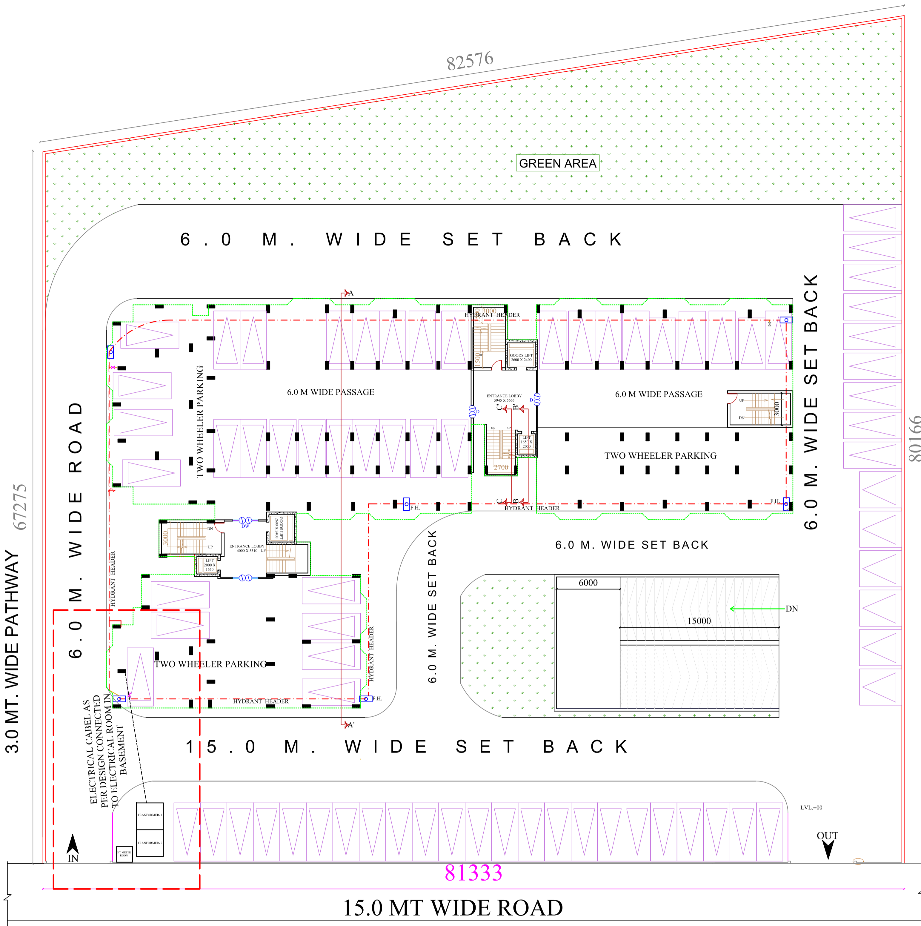
GROUND [STILT] FLOOR PLAN SCALE 1:200
