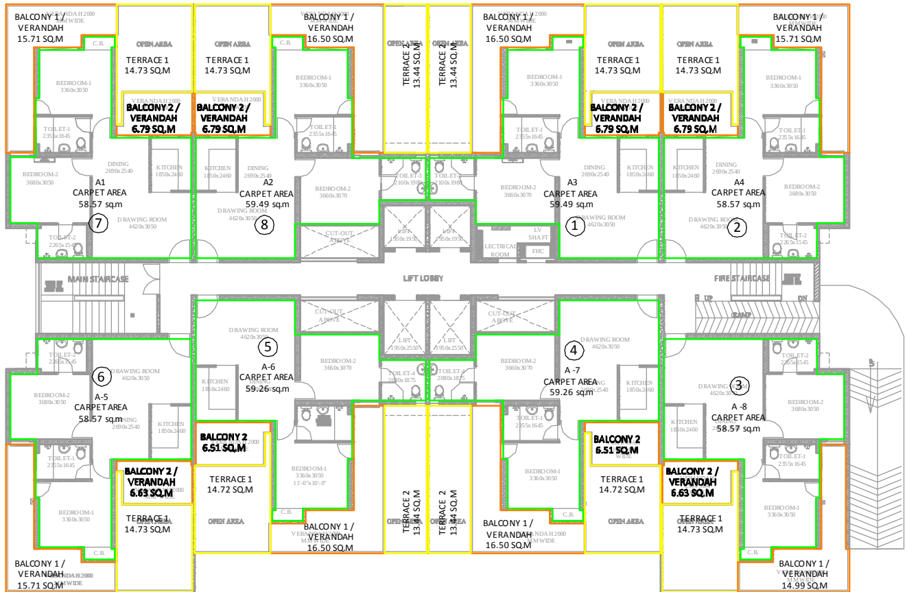
PODIUM FLOOR PLAN
