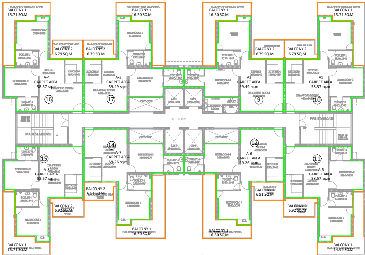
TYPICAL FLOOR PLAN (1ST TO 32nd FLOOR)
