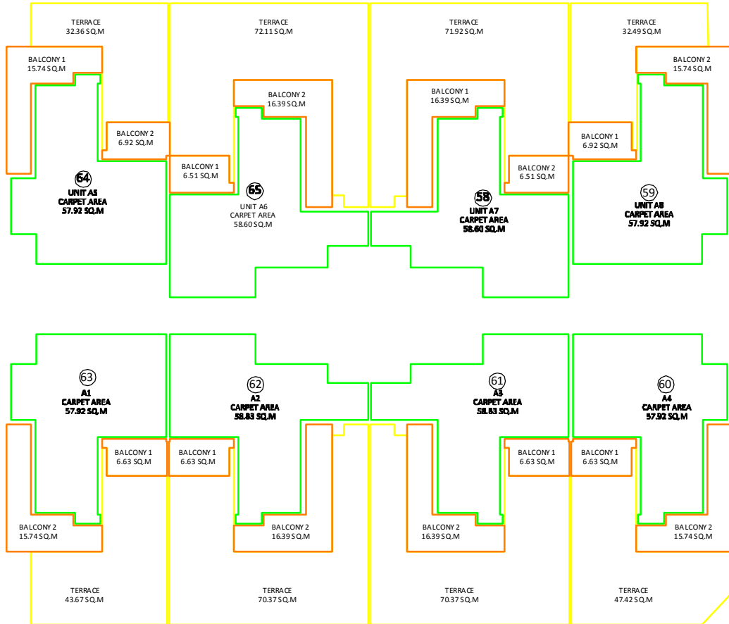
1st FLOOR AREA DETAIL
