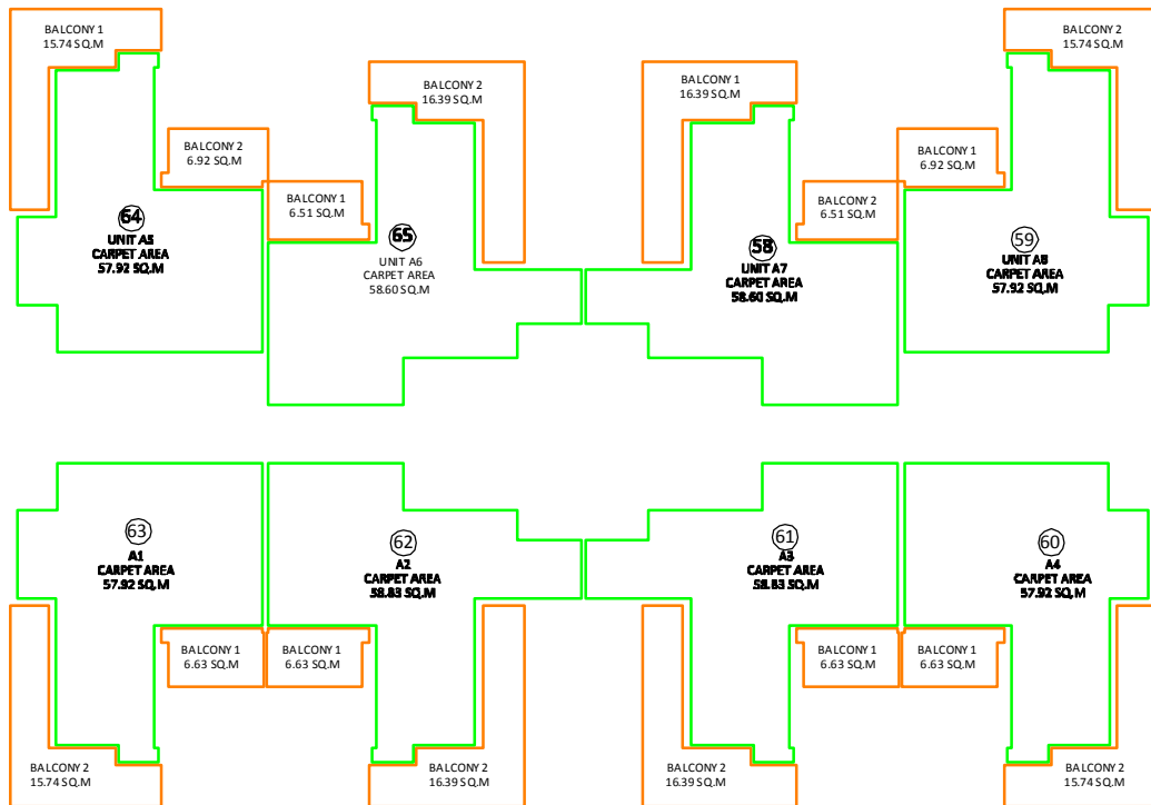
TYPICAL FLOOR AREA DETAIL (2nd TO 21st FLOOR)
