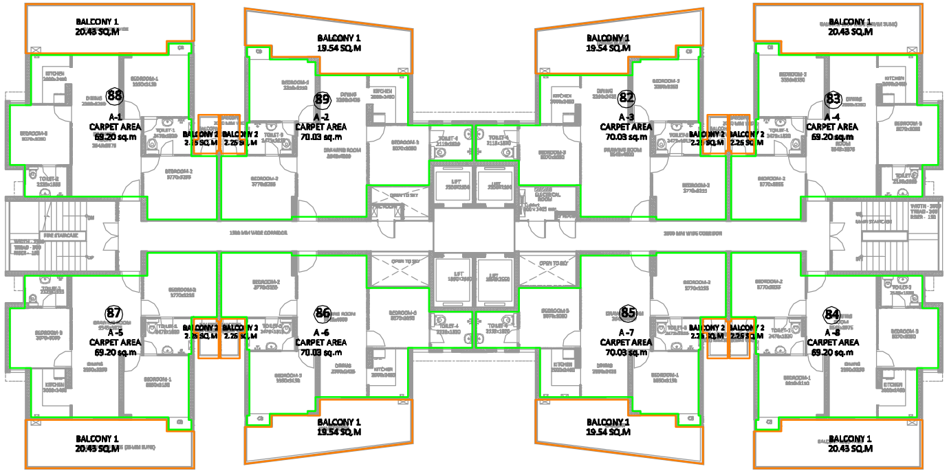
TYPICAL FLOOR PLAN (1st TO 32nd FLOOR )
