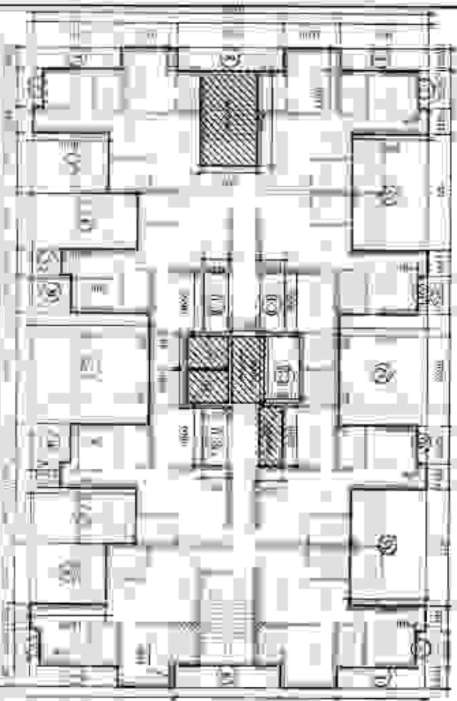
TYPICAL FLOOR SUPERIMPOSED PLAN
