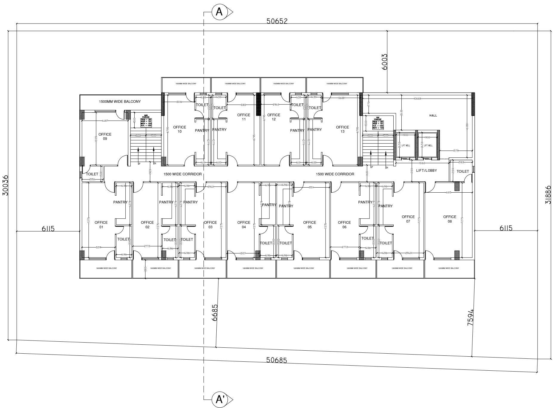
FOURTH & FIFTH FLOOR PLAN
