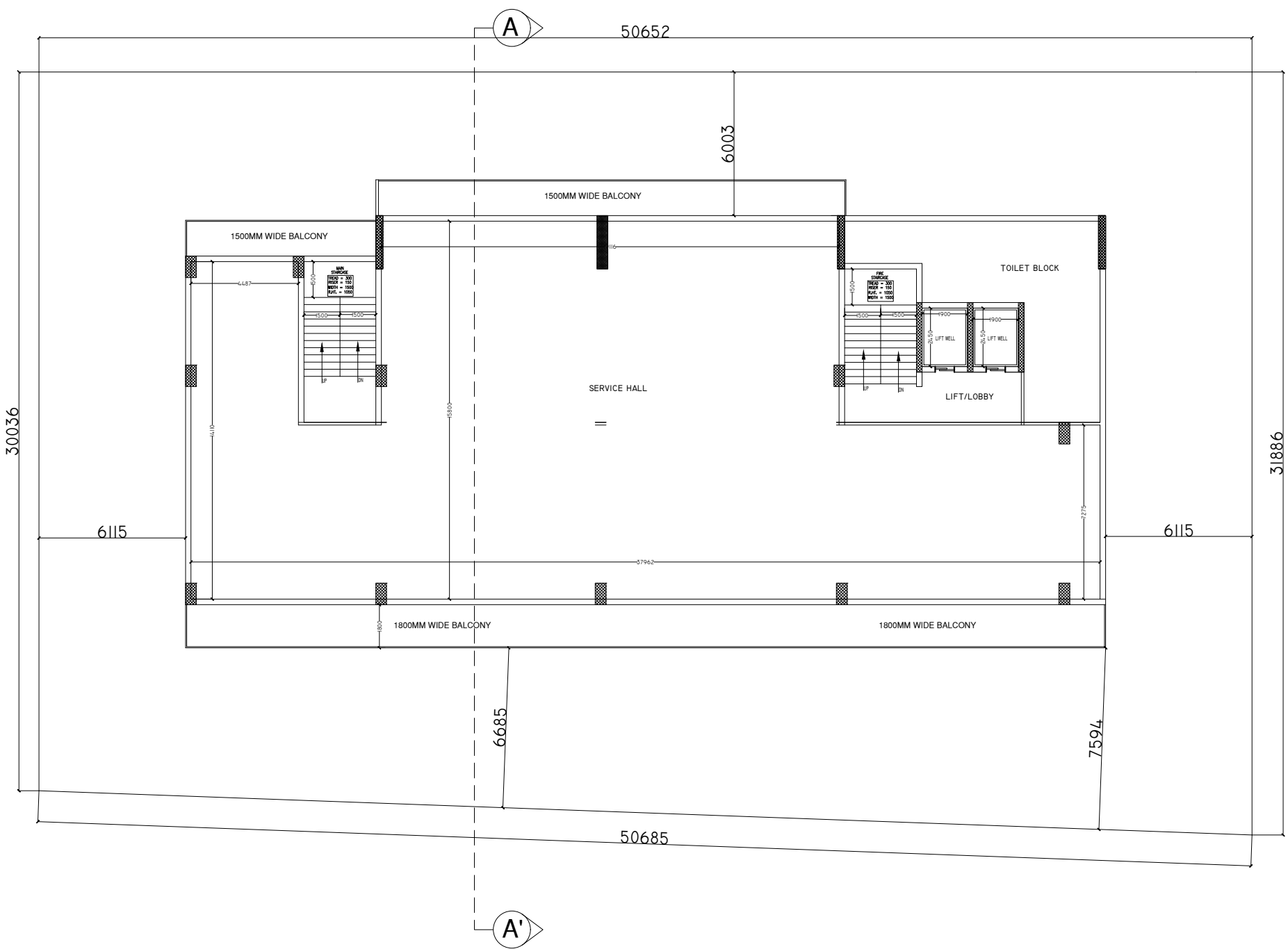
3rd FLOOR (SERVICE FLOOR) PLAN
