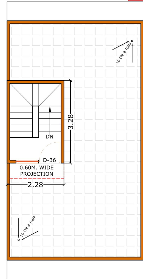
TERRACE PLAN
