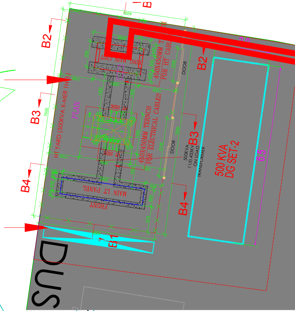
ELECTRICAL SUBSTATION-1
