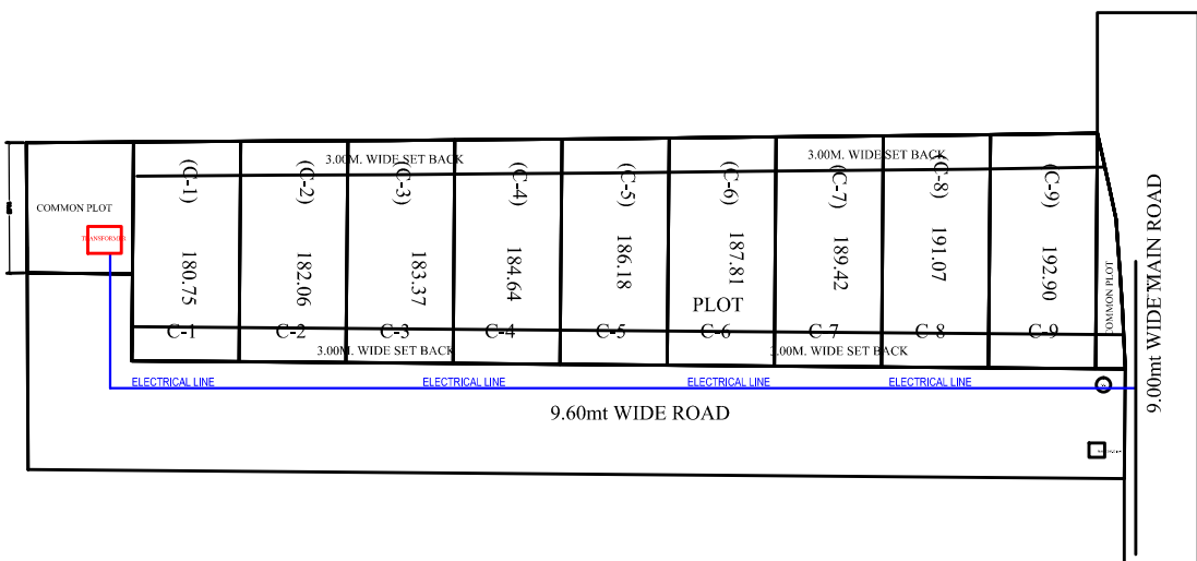
ELECTRICAL PLAN
