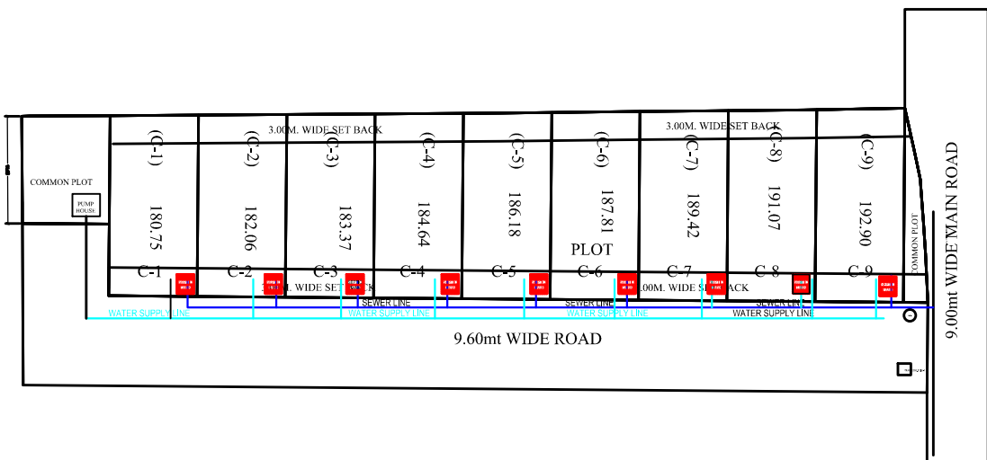
SERVICE PLAN
