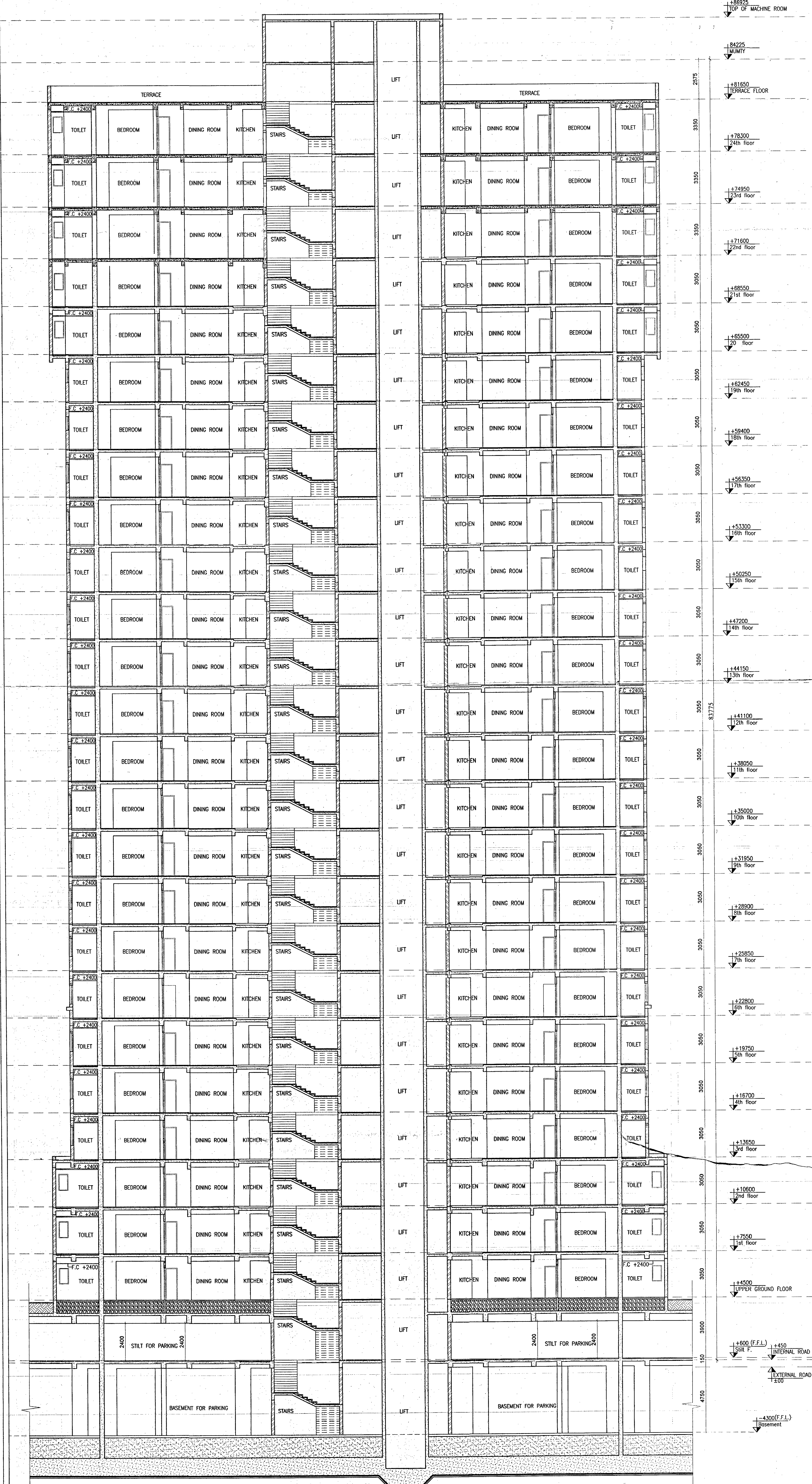
SECTION BB
