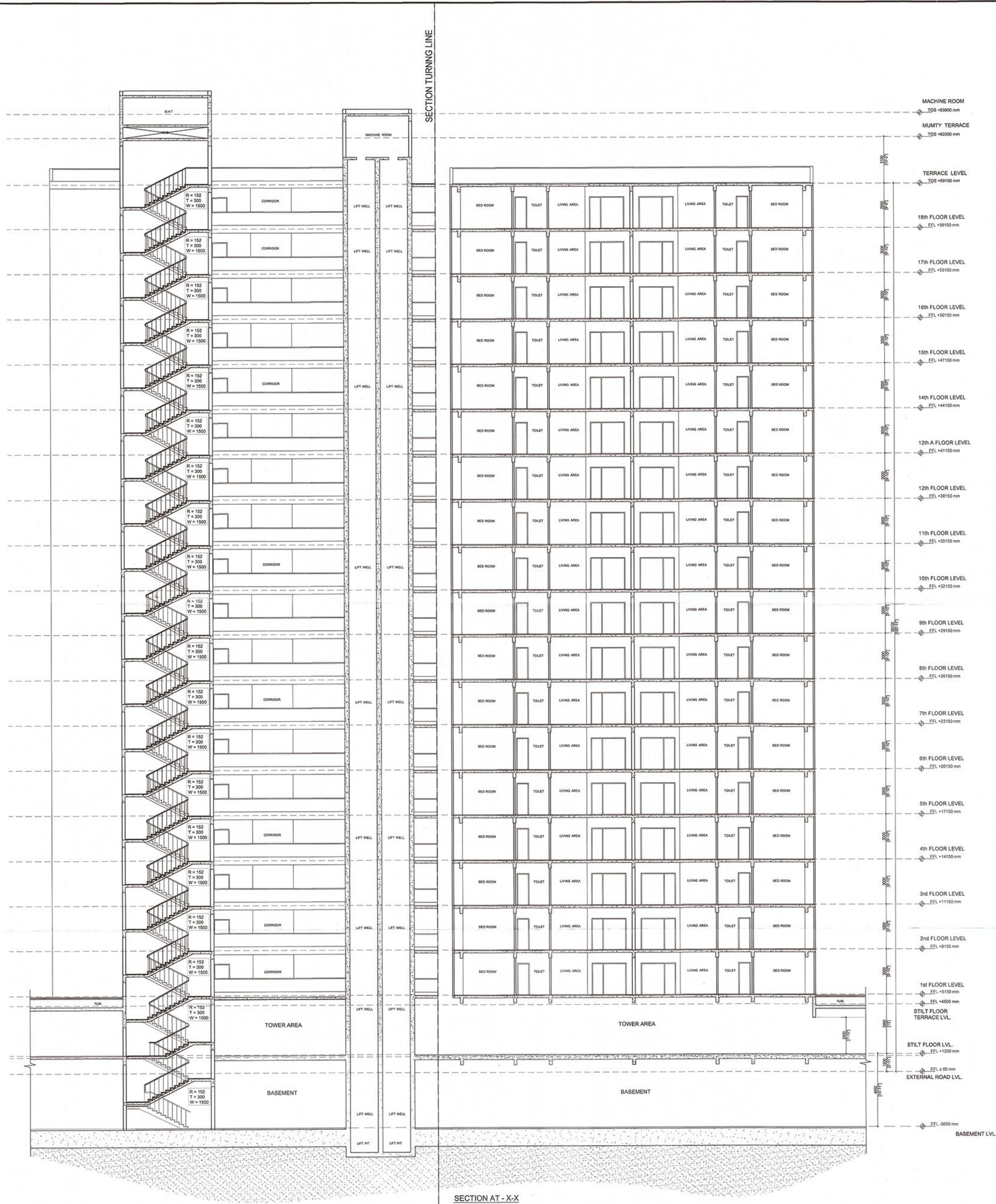
SECTION AT - X-X
