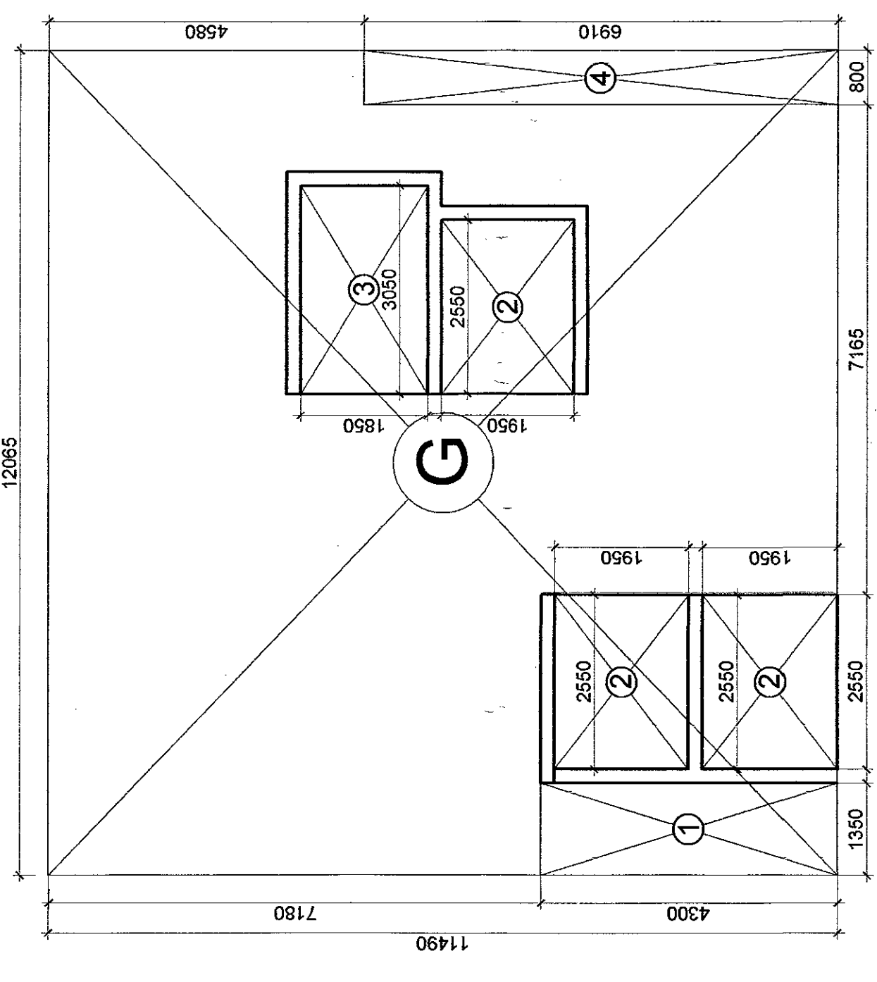
AREA DIAGRAM TERRACE
