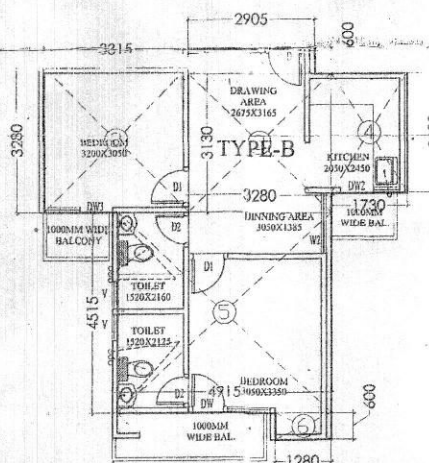
(TYPE-B DETAIL)
