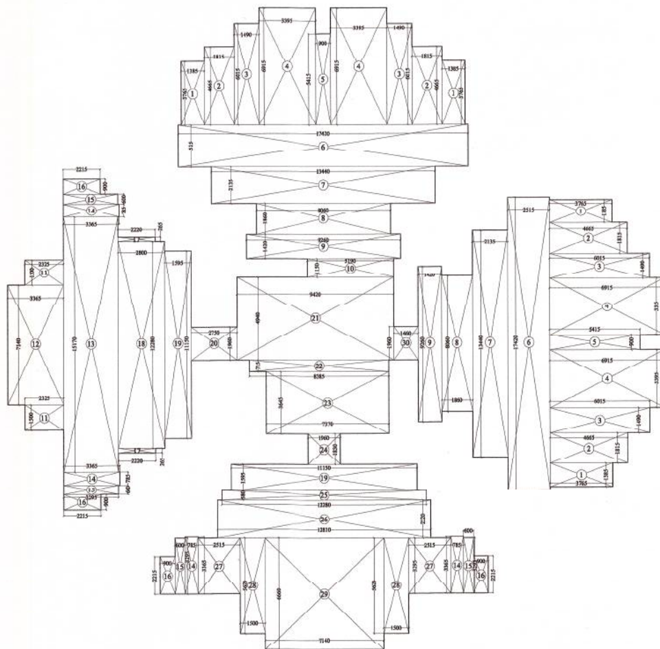
TOTAL STILT AREA DETAIL OF STILT/PODIUM FLOOR
