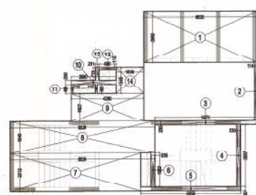
F.A.R. AREA DETAIL OF STILT/PODIUM FLOOR
