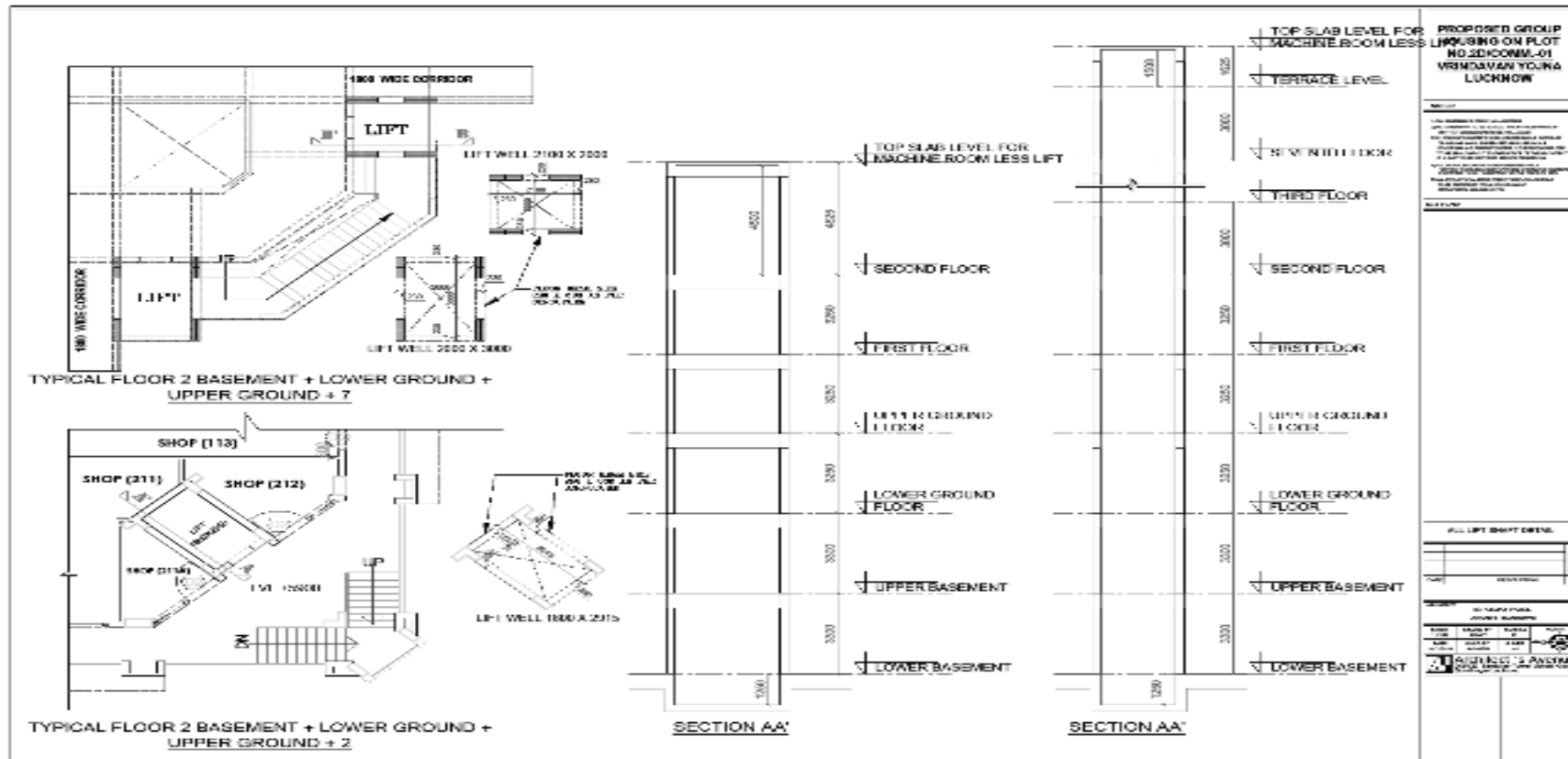
SANJAR GOLD_ALL LIFT SHAFT DETAIL_19122018
