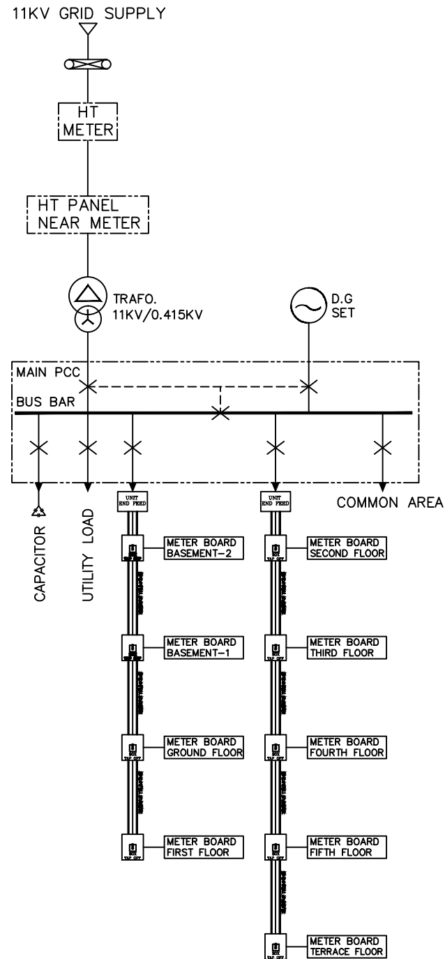
ELECTRICAL SUPPLY SCHEMATIC DIAGRAM
