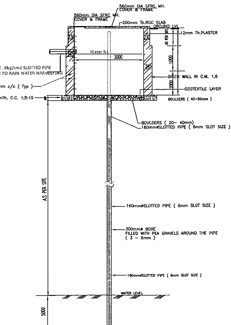
SECTION-R.R. 160mm dia. P.V.C. SLOTTED PIPE ( 6mm SLOT SIZE )
