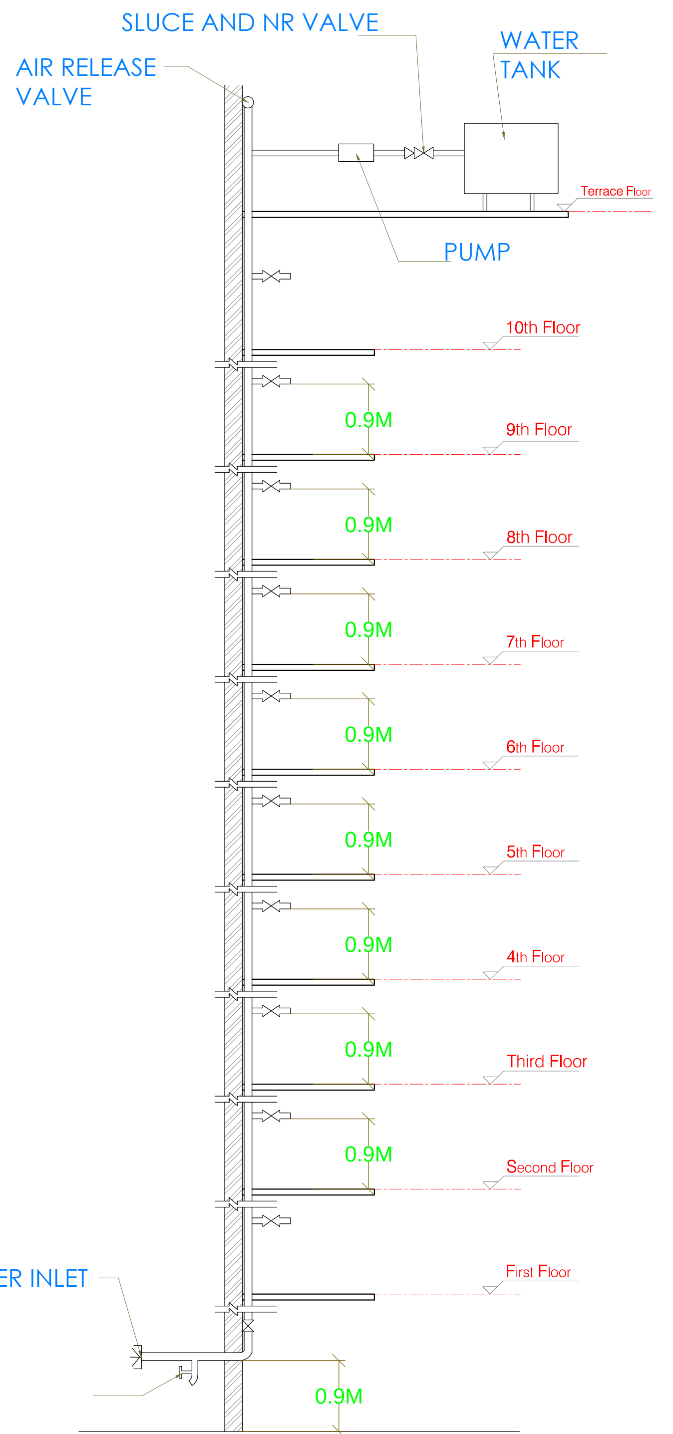
TYPICAL ARRANGEMENT OF DOWN-COMER FOR BUILDING
