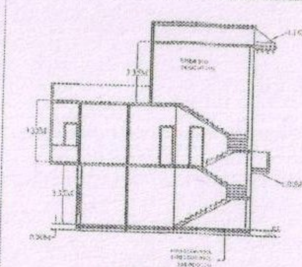
SECTION H-H
