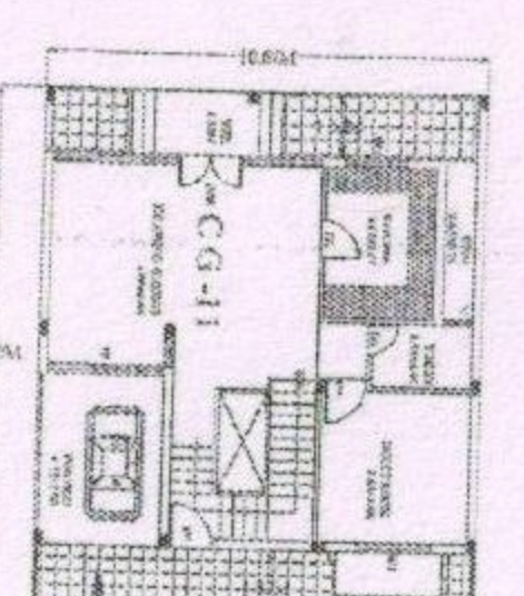
SECTION M-M
