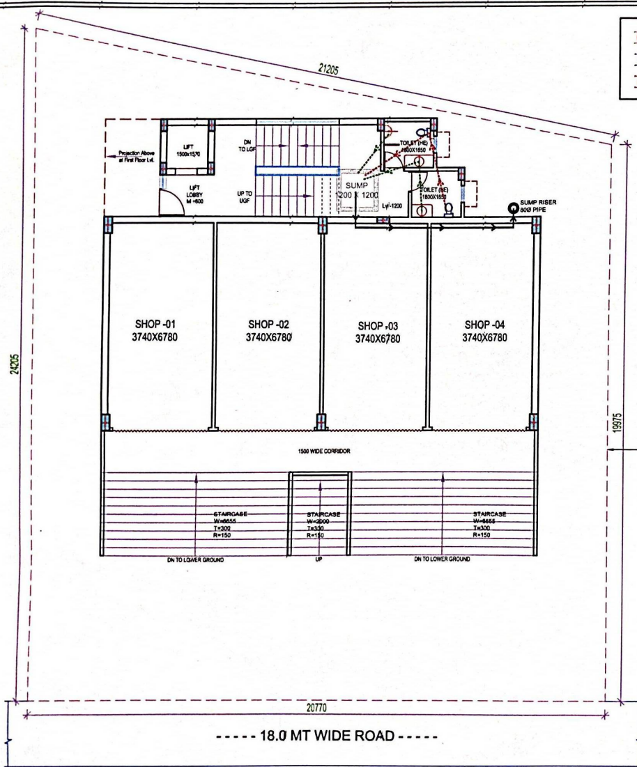
LOWER GROUND FLOOR PLAN
