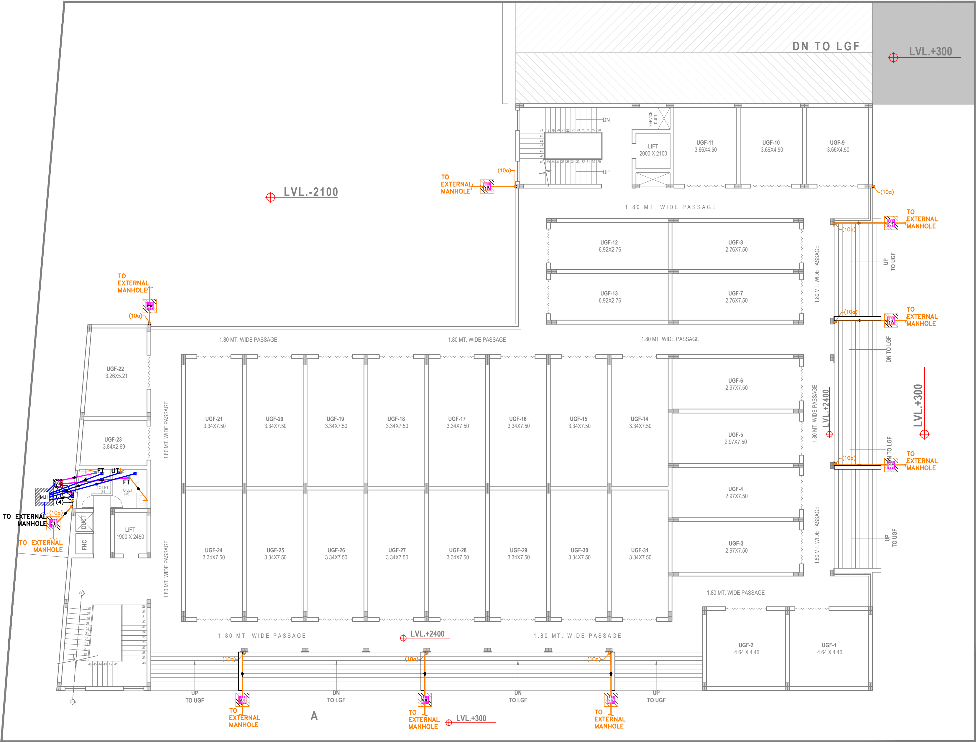
PLUMBING DRAWING DRAINAGE SYSTEM UPPER GROUND FLOOR PLAN
