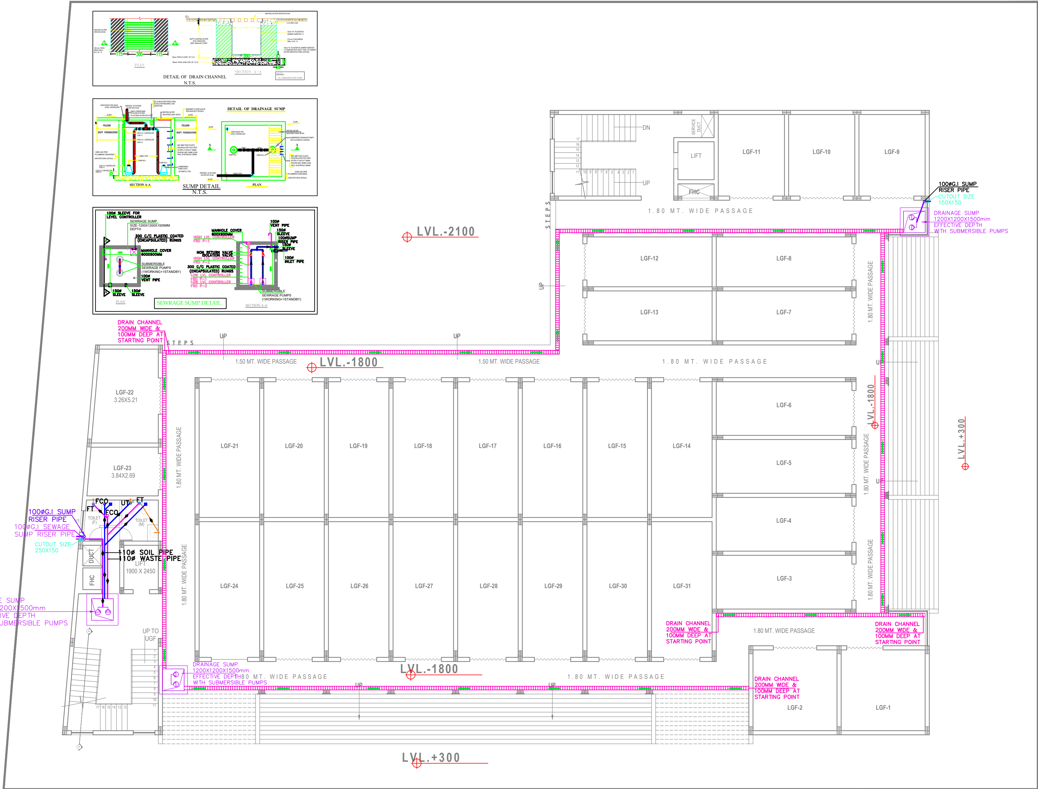
PLUMBING DRAWING DRAINAGE SYSTEM LOWER GROUND FLOOR PLAN
