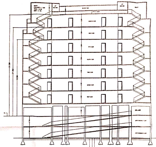
SECTION ON 'X-X'
