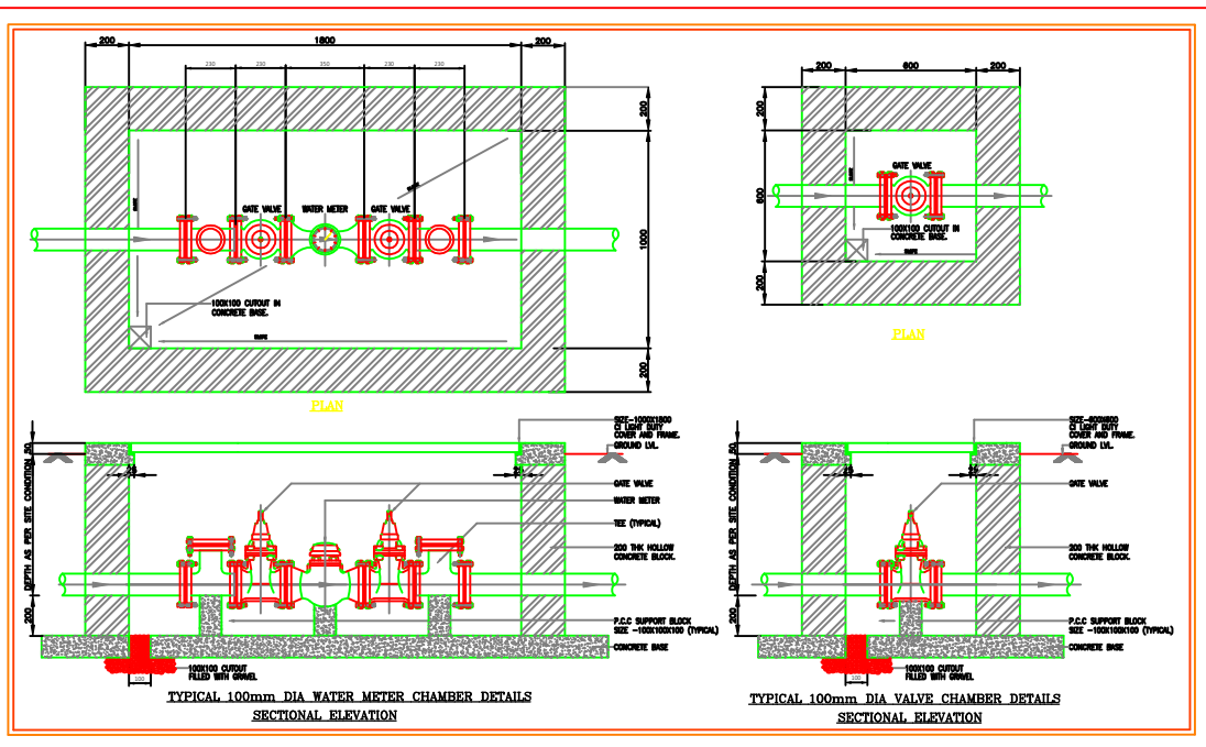
TYPICAL VALVE CHAMBER DETAILS (QASR AL ALAM)
