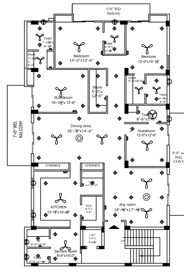
TYPICAL FLOOR PLAN OF BLOCK C
