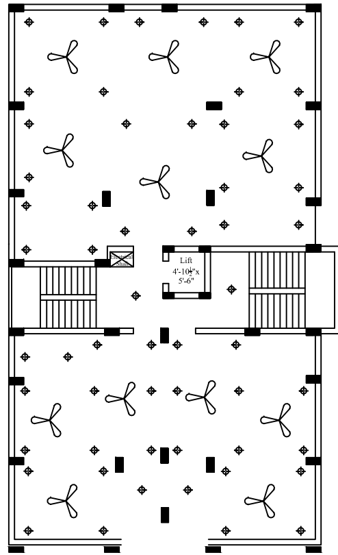
BASEMENT FLOOR PARKING PLAN OF BLOCK D
