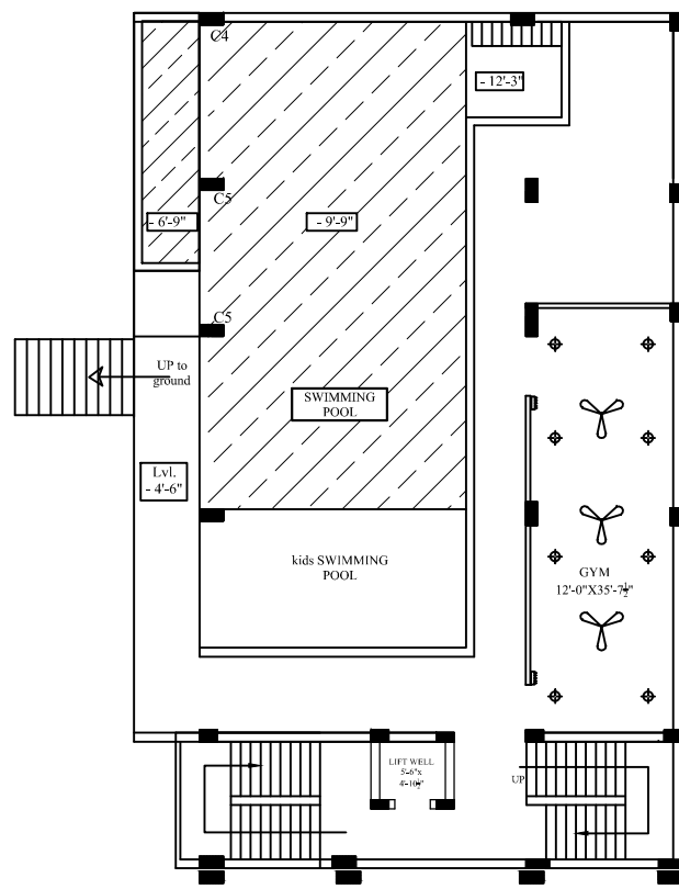
BASEMENT PLAN OF BLOCK C
