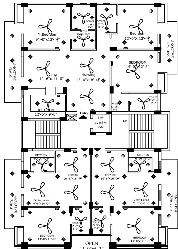
TYPICAL PLAN OF BLOCK D
