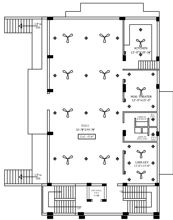
STILT FLOOR PLAN OF BLOCK C
