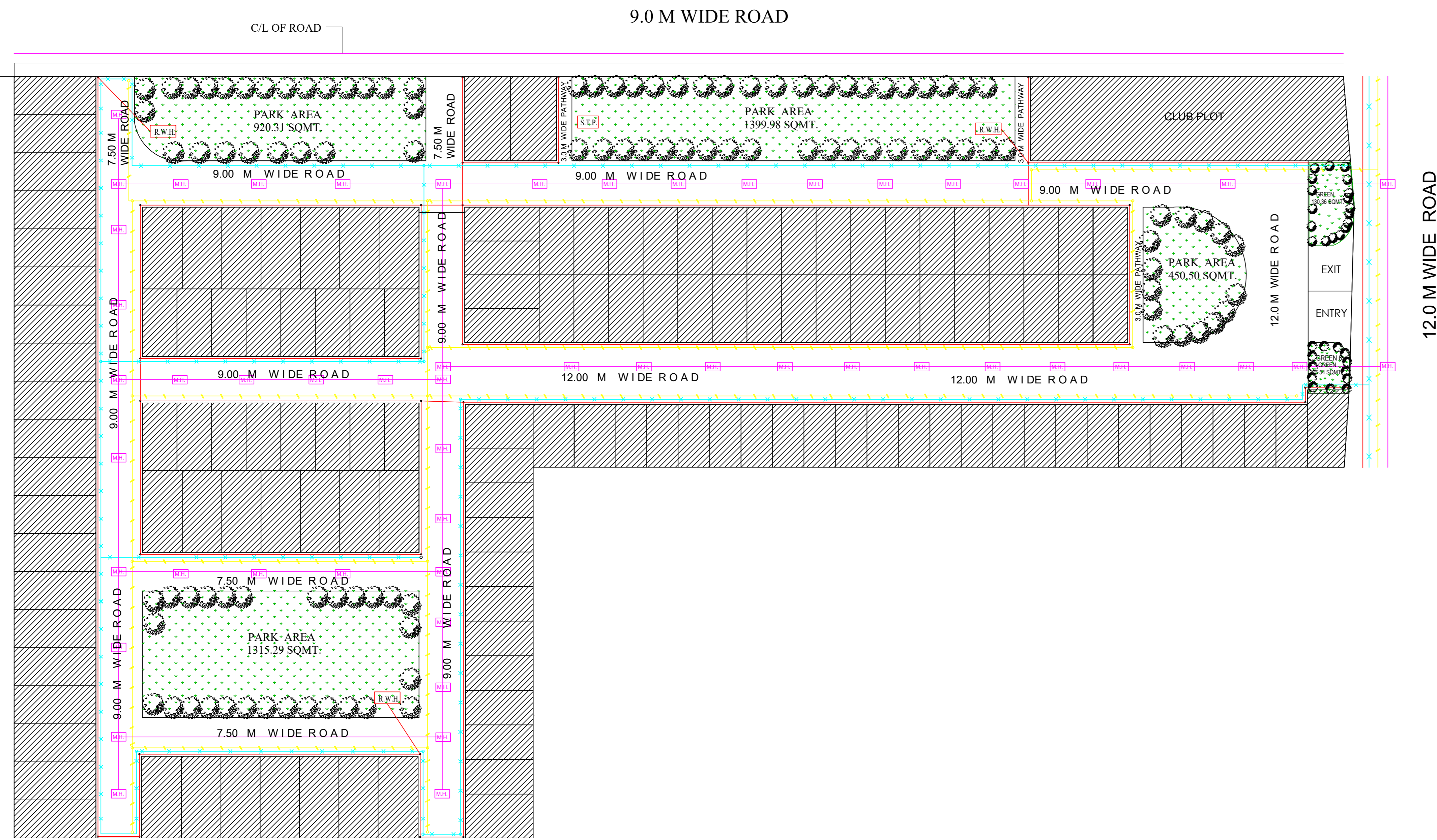
LANDSCAPE AND SERVICE PLAN SCALE = 1:200
