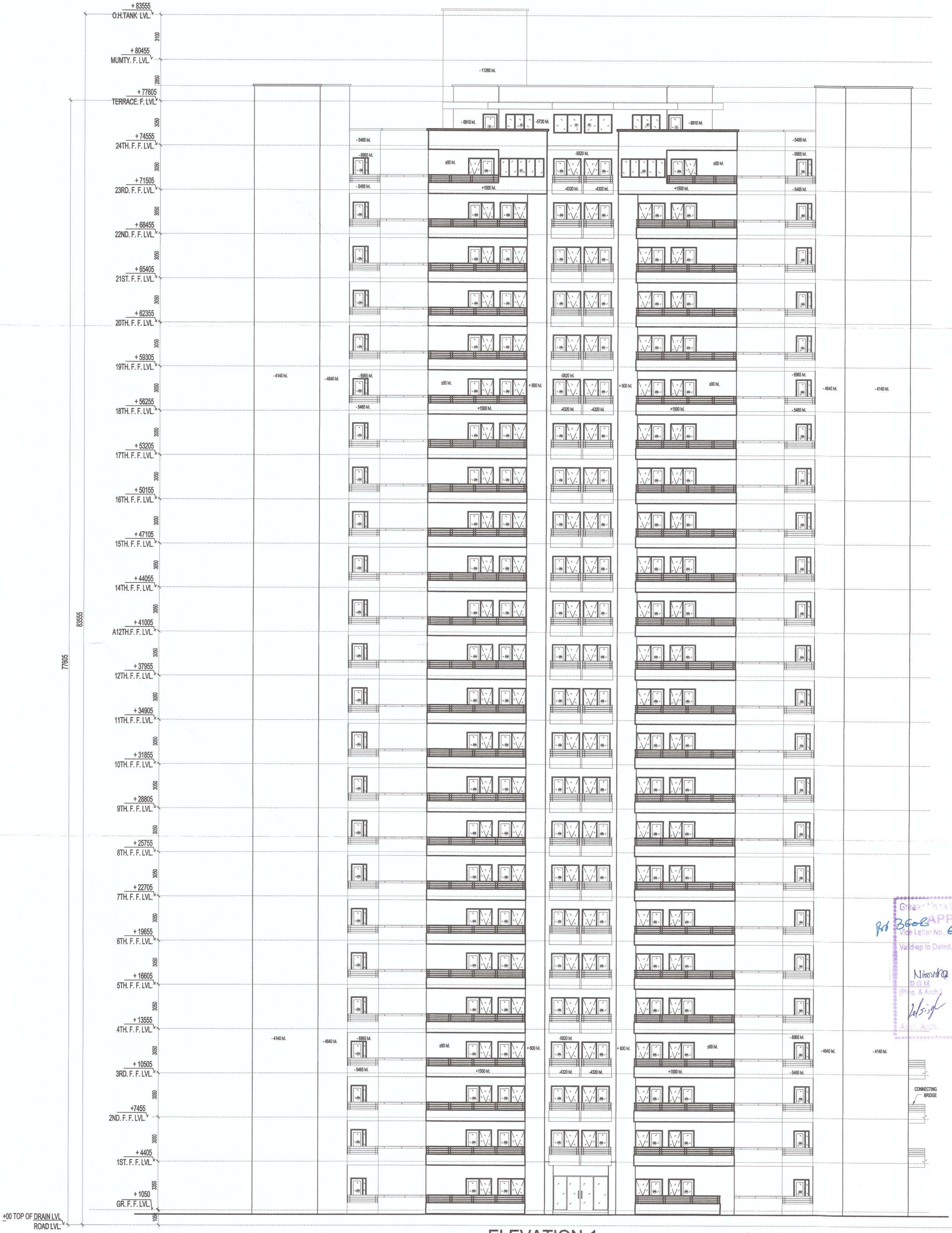
ELEVATION-1
