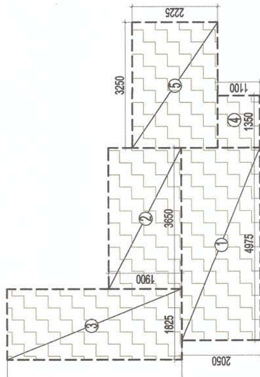
AREA DIAGRAM FOR TYPE-D UNIT
