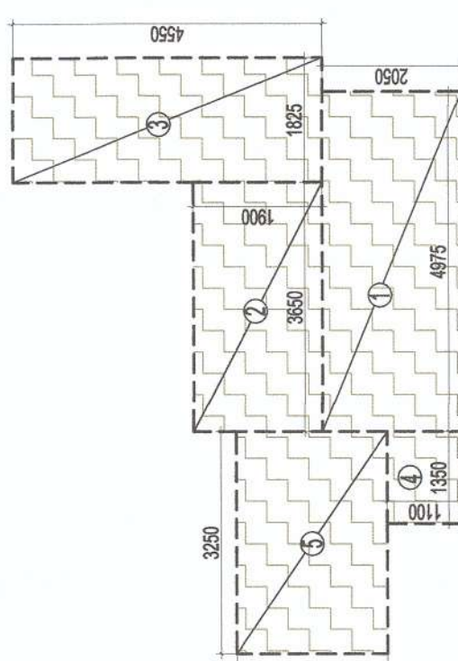
AREA DIAGRAM FOR TYPE-B UNIT
