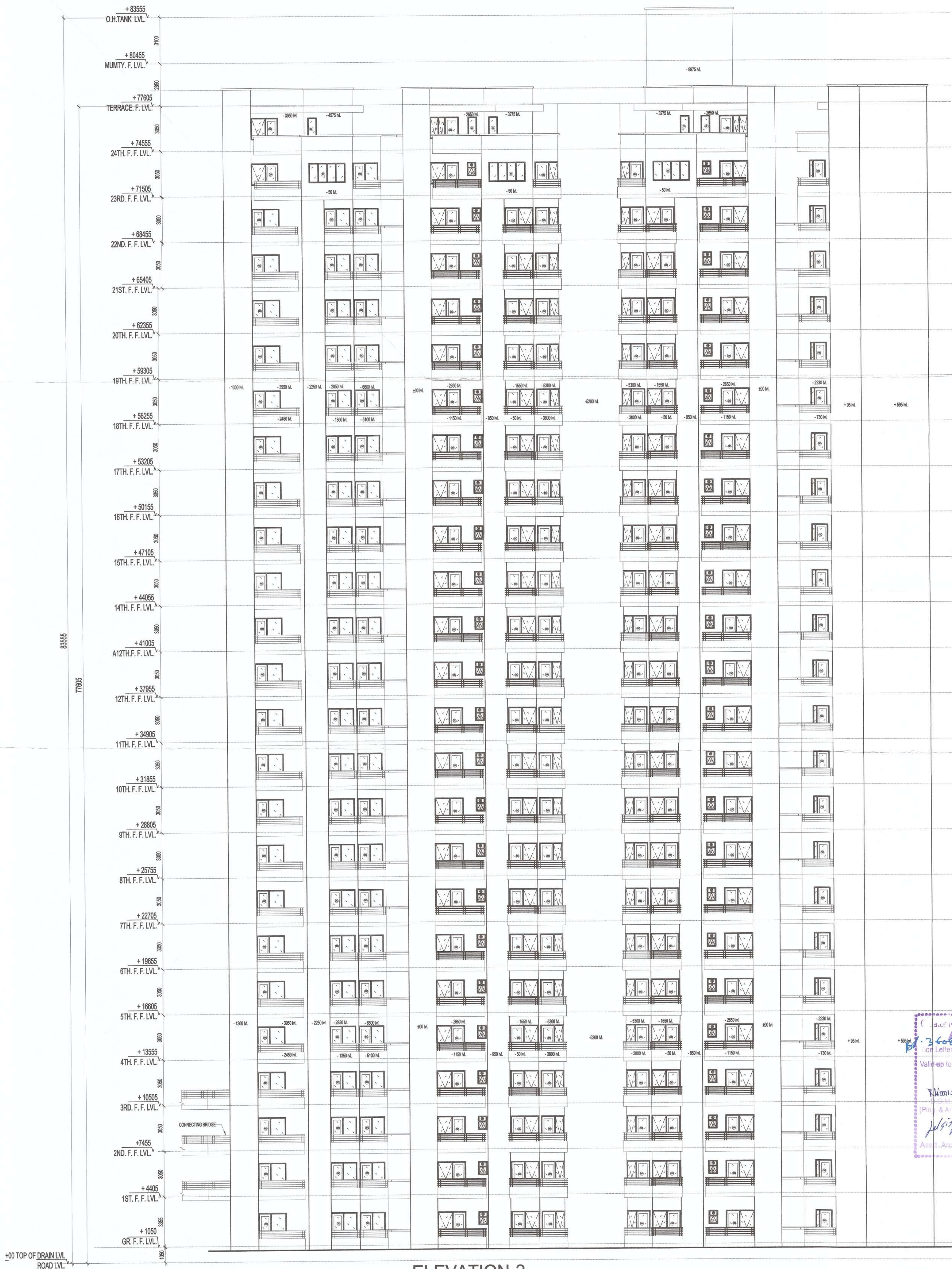
ELEVATION-2
