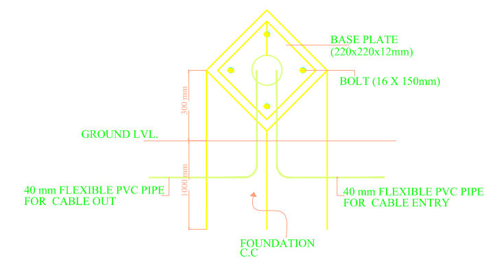
DETAIL AT-A
