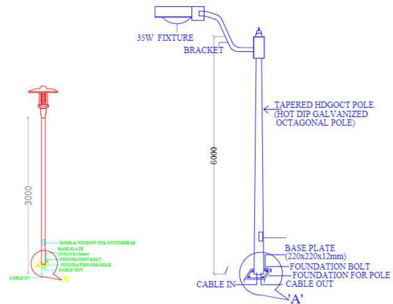
(POCKET - 1) SERVICES PLAN SHOWING
