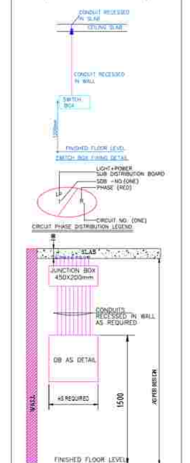
TYPICAL DETAIL OF DB FIXING
