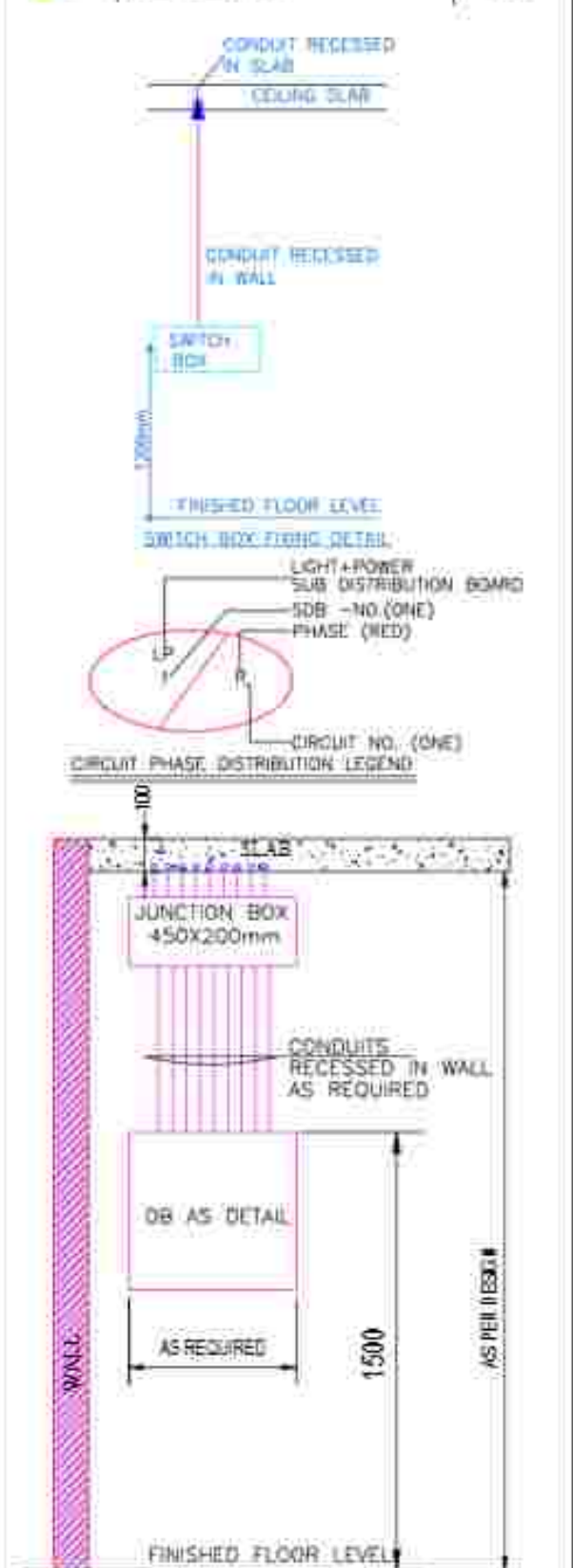
TYPICAL DETAIL OF DB FIXING
