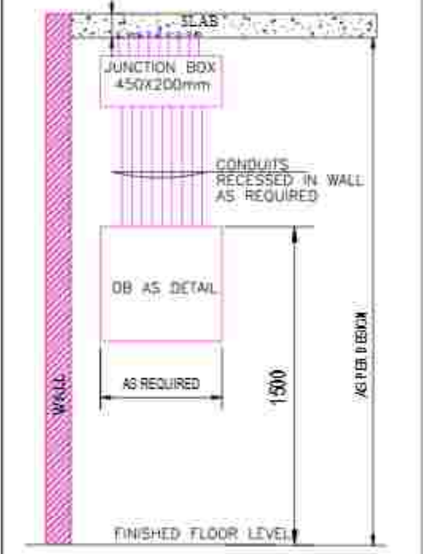
TYPICAL DETAIL OF DB FIXING
