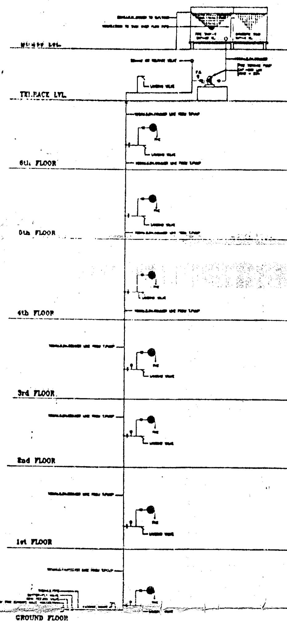
FIRE FIGHTING SYSTEM DIAGRAM
