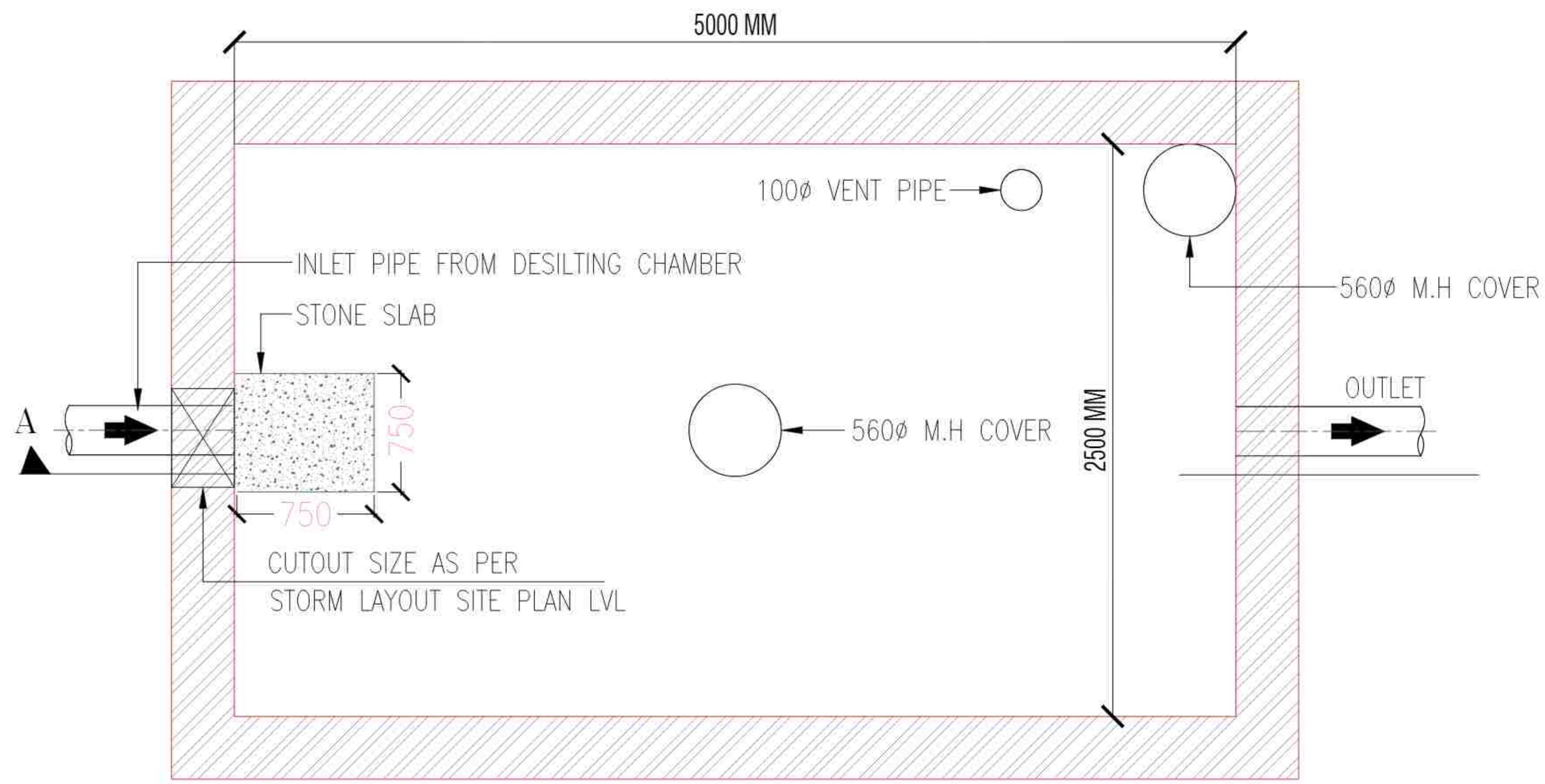
PLAN OF RECHARGE WELL
