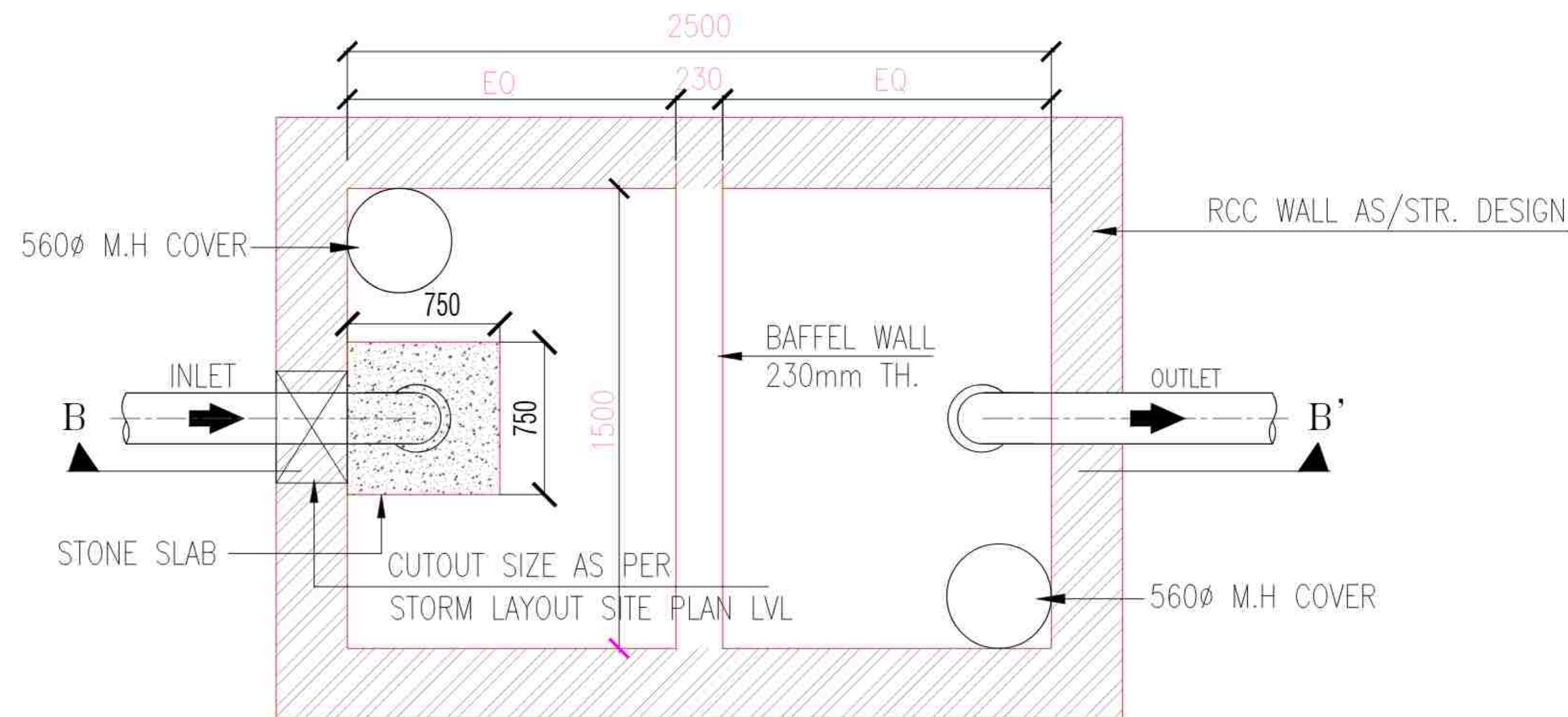
PLAN OF DESILTING CHAMBER
