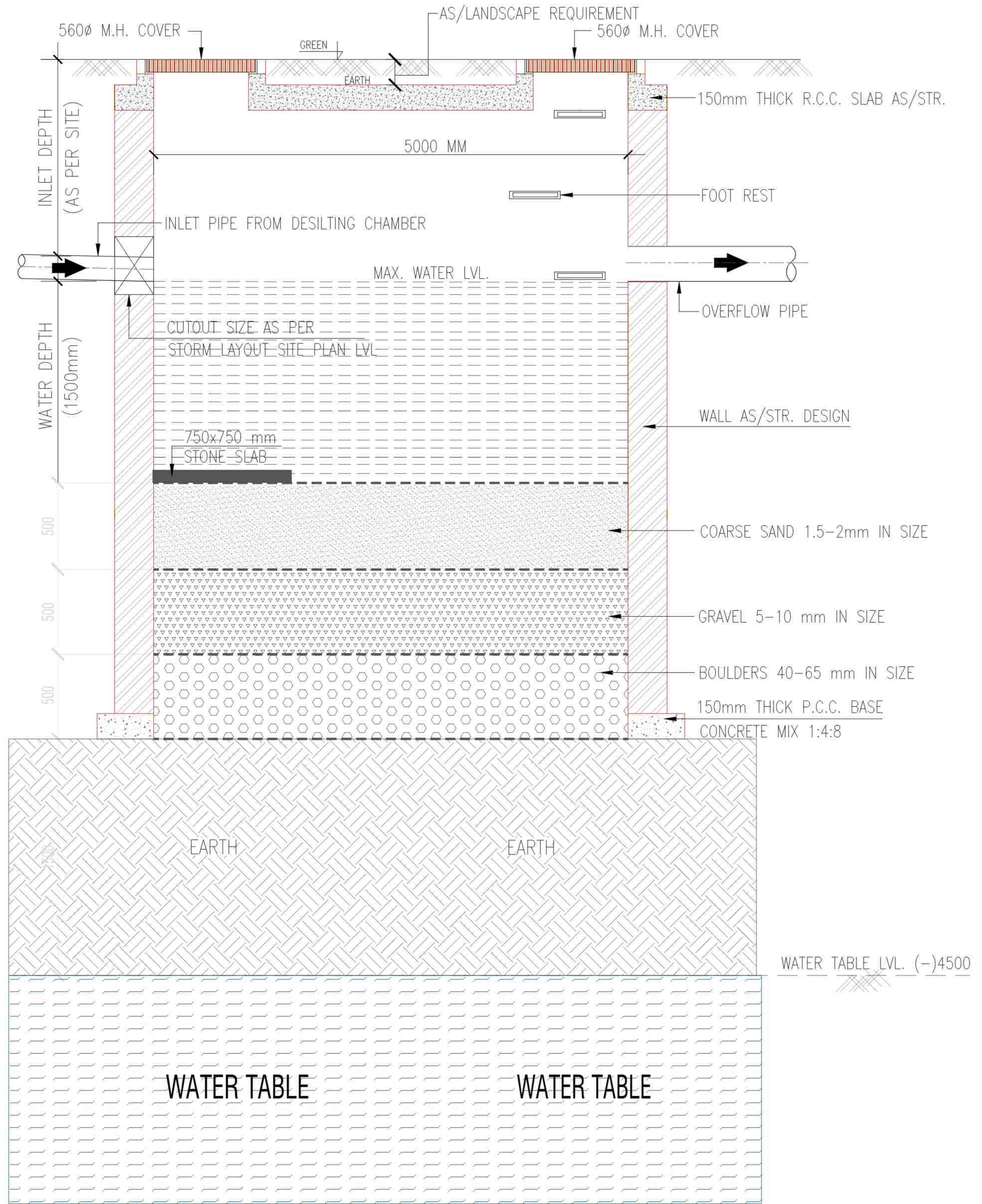
SECTION-A-A'
