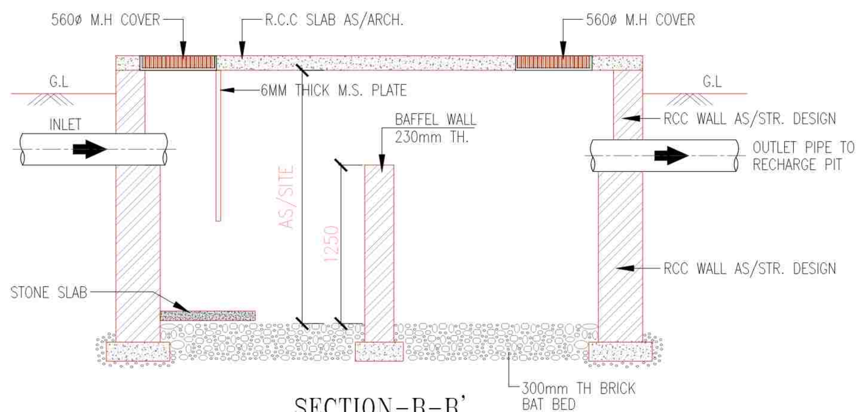
SECTION-B-B'
