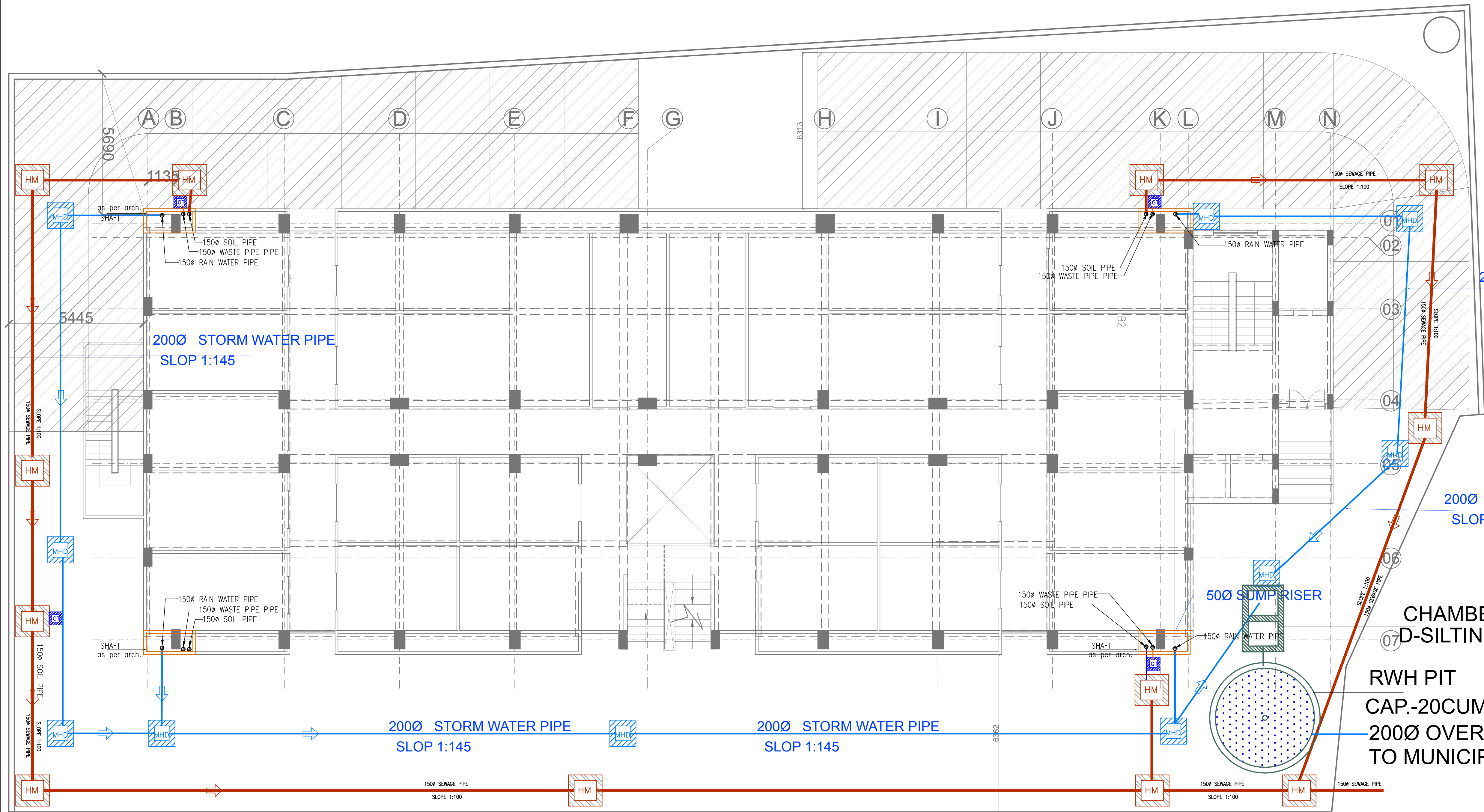
UPPER GROUND FLOOR PLAN
